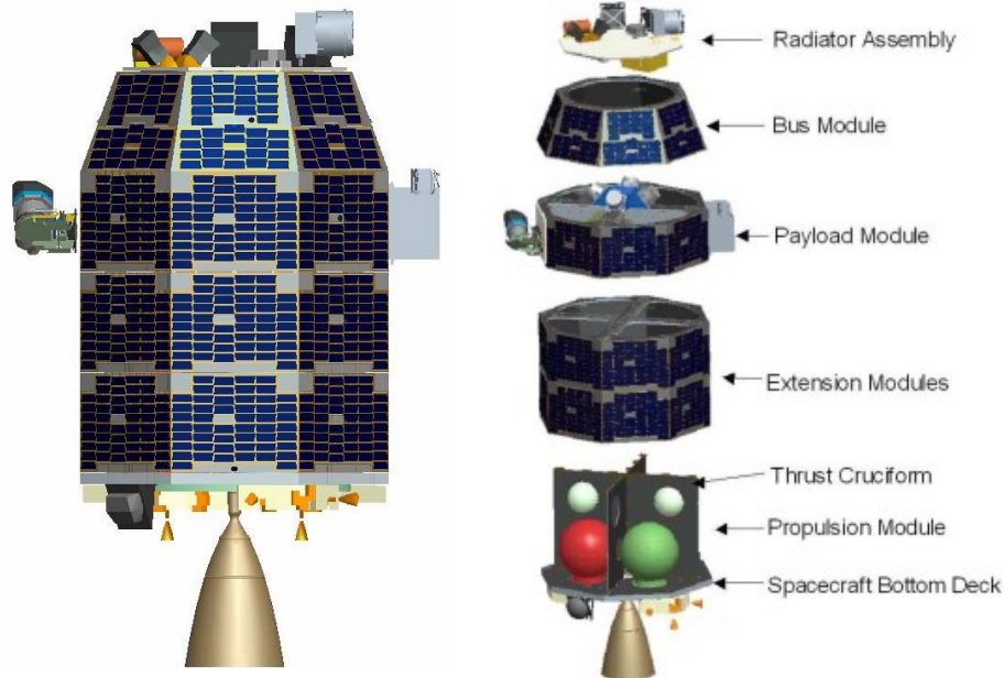
Figure 3-1: LADEE major structural components and layout
