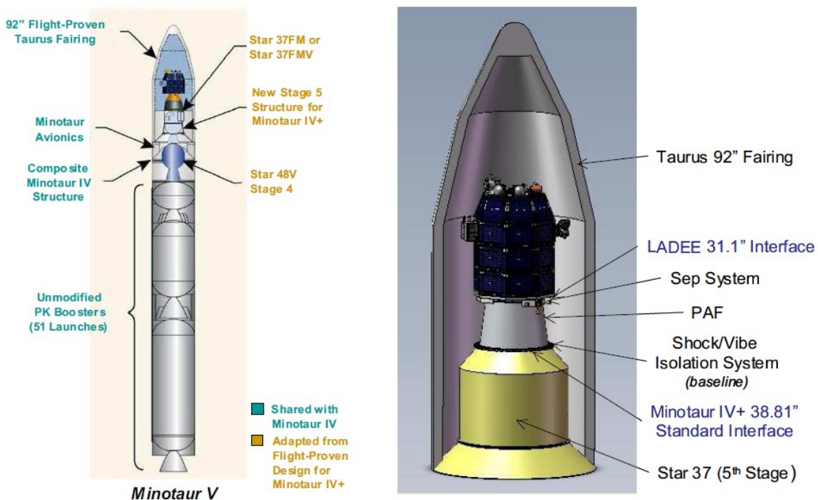
Figure 2-1: LADEE launch vehicle and configuration
