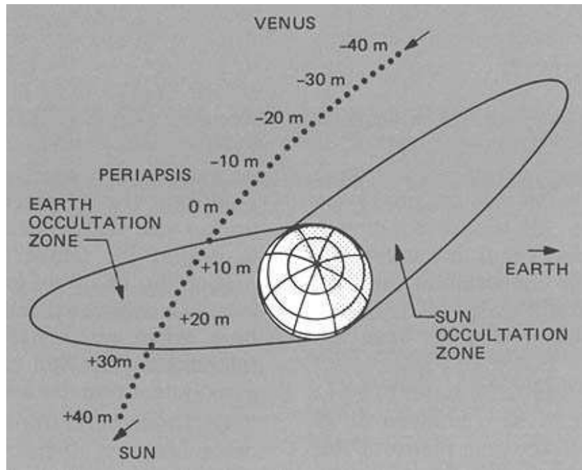
Fig. 5-12. A further trajectory correction maneuver and Mariner 10 was all set for its encounter with Venus.
