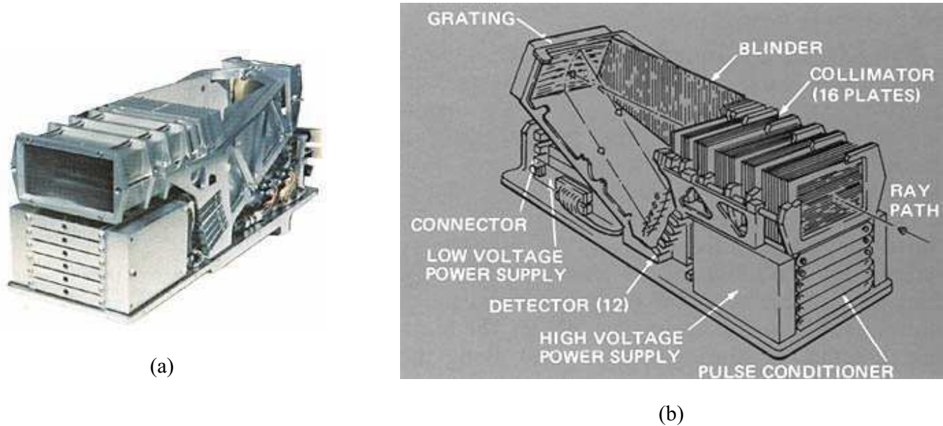
Fig. 3-8. The second ultraviolet instrument, an airglow experiment, looked for radiation from the planet directly, scanning through the atmosphere on both bright and dark limbs to search for atmospheric gases. Shown here are (a) a photograph of the instrument and (b) a cutaway view.
