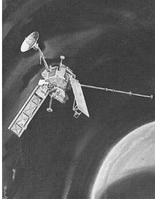
Fig. 4-1. One method of safeguarding the solar panels from overheating as Mariner approached closer to the Sun was to tilt them into a V-configuration.
