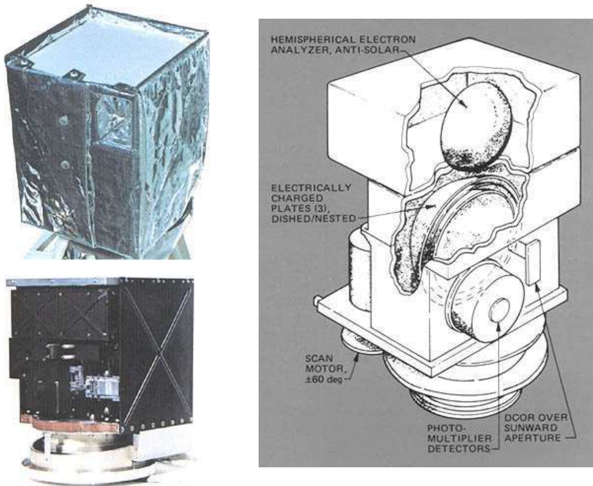
Fig. 3-4. A plasma science experiment relied upon two detectors mounted on a scan platform. The scanning electrostatic analyzer consisted of three hemispherical plates directed toward the Sun to measure incoming electrons and positive ions.
