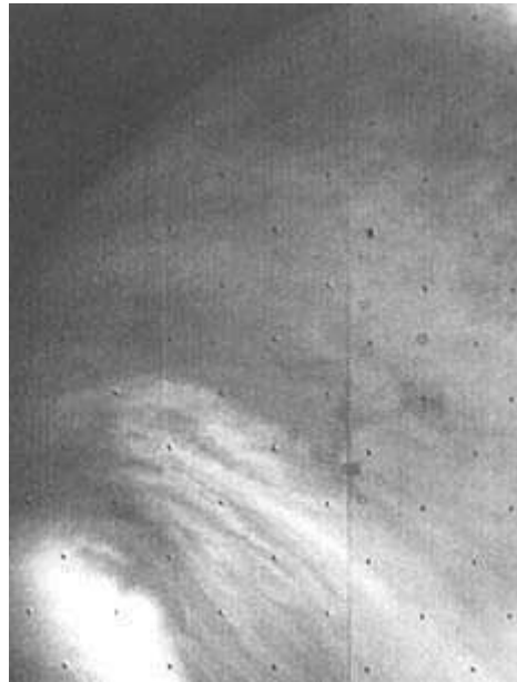
Fig. 6-4. When ultraviolet photographs of Venus came back to Earth as Mariner sped away from Venus, they showed surprising details of atmospheric patterns. This view of the southern hemisphere taken one day after closest approach reveals spiral-like markings and streamline flows. The picture, part of a 36-frame full-planet mosaic, was taken at 10:15 a.m. PDT, February 6, from a range of about 725,000 km (450,000 ml). The pattern of dots is on the face of the vidicon tube and is used to calibrate the image.
