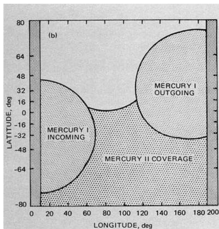
Fig. 8-1. The second encounter with Mercury allowed Mariner 10 to fly by the planet on the sunlit side, thereby filling in the missing areas between the two sections photographed at the first encounter. This second encounter took place on September 21, 1974. Additionally, in this encounter Mariner was able to obtain good views of the south polar region of Mercury. An artist's concept of the second flyby is shown in (a); (b) shows the added coverage obtained of the illuminated hemisphere.
