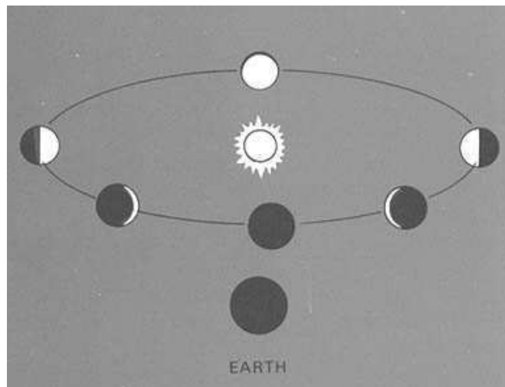
Fig. 1-4. Galileo discovered that Venus, seen through a telescope, shows phases like those of the Moon.
