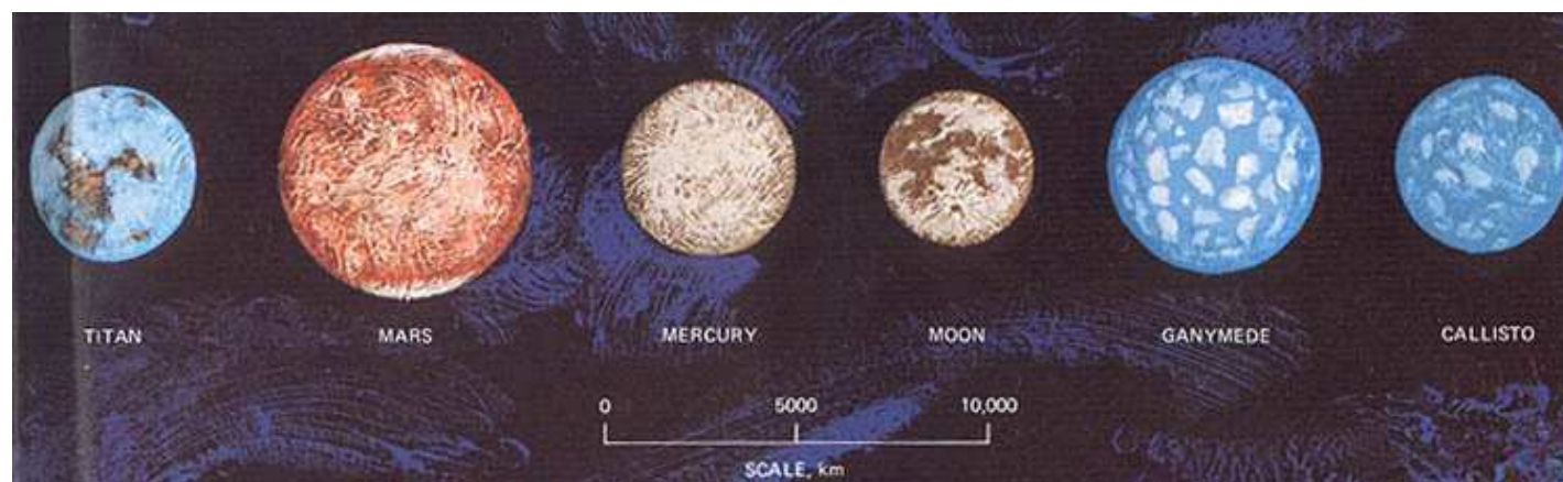
Fig. 1-7. In comparison, Mercury is between the Moon and Mars in size. Some satellites of the outer planets are equally as large.
