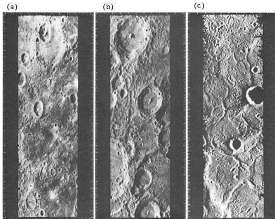
Fig. 8-10. High-resolution pictures, each only a quarter frame, were obtained at the third encounter, Mercury lilt In the upper portion of (a), which was taken from a distance of 67,000 km (41,500 mi) on March 16, 1975, a multiple impact feature of three craters of different sizes nested within the largest is shown. The smallest crater is about 15 km (9 mi) in diameter. The bright feature at the bottom was caused by impact of a meteorite; it is a fresh crater. Craters ranging in size from 30 to 50 km (18.5 to 31 mi) are shown in (b). It was taken at a distance of 65,000 km (40,000 mi), one hour and 45 min before closest approach. The fractured and ridged plains of the floor of the Caloris basin are shown in (c). The area is located at 31°N latitude and 183°W longitude. The picture was taken at a range of 19,000 km (11,800 mi), 34 min after the spacecraft swept past Mercury for the third and final encounter.
