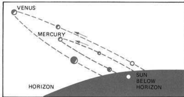
Fig. 1-2. Because Mercury and Venus orbit the Sun within Earth's orbit, they stay close to the Sun in the sky as seen from Earth. At their greatest angular distance from the Sun they are said to be at elongation. Here the two planets are shown at eastern elongation; they set after the Sun and appear as evening stars.
