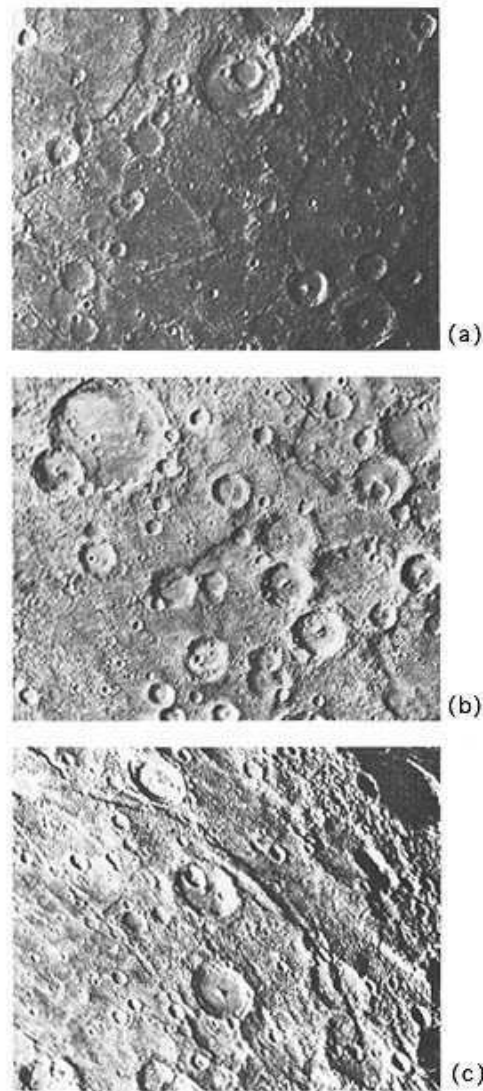
Fig. 8-5. The new pictures were fantastic. A southern hemisphere area of heavily cratered terrain (460 by 650 km, 285 by 400 mi) on which a prominent scarp extends several hundreds of kilometers at the upper left is shown in (a). The smallest details measure about 1.7 km (1 mi). Another densely cratered region containing a scarp which rises about two km (7500 ft) above the surrounding area is shown in (b). The scarp shown in (c) is more than 300 km (185 mi) long.
