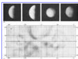
Fig. 1-8. Mercury, too, reveals few details, not because of clouds but because of the planet's small size, its distance from the Earth, and its closeness to the Sun. Photographs (a) show only indistinct shadings, and maps (b) made on the basis of observations from Earth are virtually useless.
