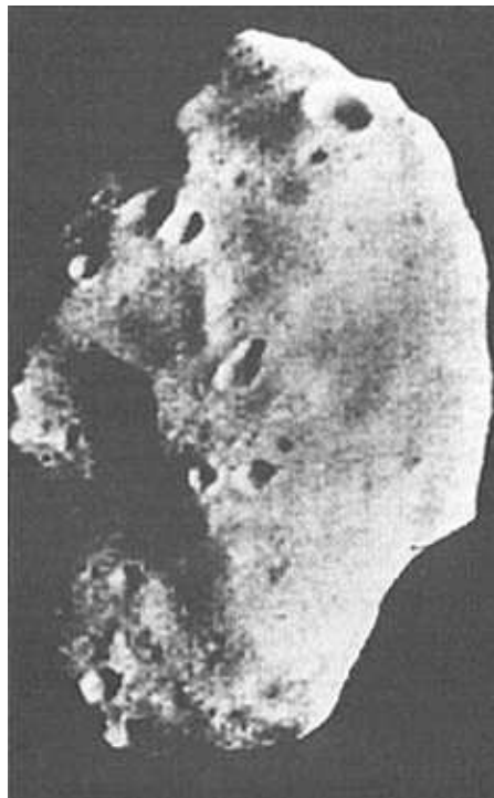
Fig. 1-5. Craters on terrestrial planets and satellites, like these revealed by a Mariner spacecraft on a satellite of Mars, are thought to be the evidence of the final stages of an accretion process that took place some 4.5 billion years ago.
