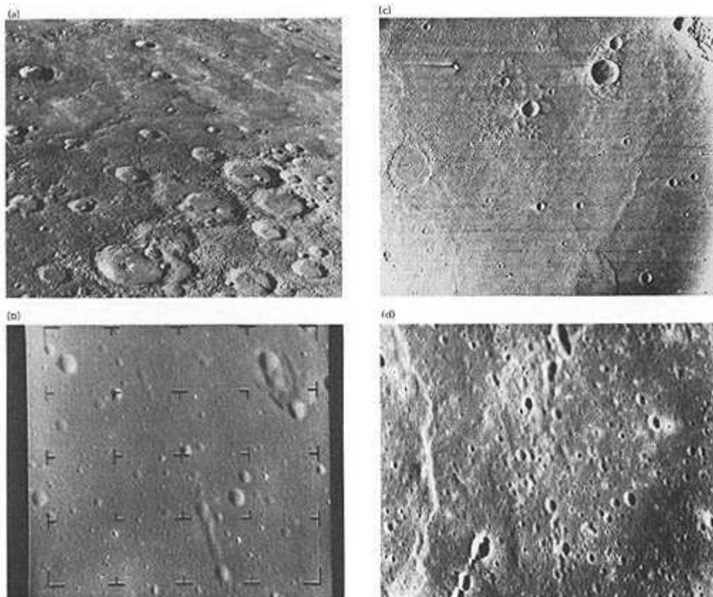
Fig. 7-15. Although superficially the plains of Mercury (a [top left]) seem similar to those of the Moon and Mars, closer inspection reveals significant differences. The Moon (b [bottom left]) shows a surface that has been saturated with ejecta and secondary impacts. Mars (c [top right]) shows a surface that has been partially smoothed by wind erosion. Mercury's surface (d [bottom right]) may not have been covered as completely with secondary craters and ejecta as has the Moon.
