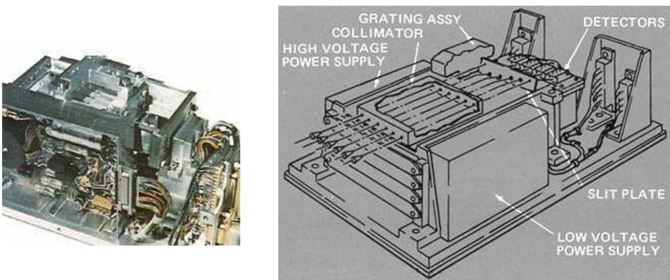
Fig. 3-7. Radiation from the planets in extreme ultraviolet provides information about certain gases such as hydrogen and helium in each planet's atmosphere. An ultraviolet experiment made use of two independent instruments. An occultation spectrometer, shown here, observed the occultation of the Sun by Mercury to probe for a Hermian atmosphere.
