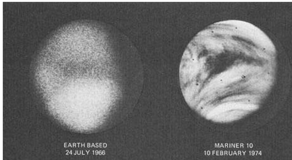
Fig. 6-5. The ultraviolet markings now photographed in great detail on Venus were obviously those seen indistinctly in ultraviolet photographs from Earth. These comparative photographs show how the gross horizontal Y-shaped marking seen from Earth is resolved into the intricate pattern of the Mariner picture on the right.
