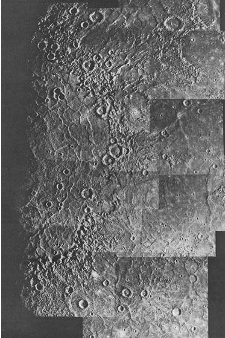
Fig. 7-12. Mariner 10 also discovered a great impact basin on Mercury that is larger than the Mare Imbrium basin on the Moon. It has been named Caloris (meaning hot) because it is located at one of the two spots on Mercury that face the Sun at perihelion, Mercury's closest approach to the Sun.
