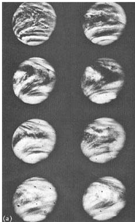
Fig. 6-7. Over the next few days, series of mosaics were constructed showing a wealth of detail in the ultraviolet markings of the planet. The relatively quick rotation of the markings was confirmed (a) and a picture built up of the cloud pattern around the entire planet (b). On the right side of (b) the pictures were taken from greater distances, so detail is lacking compared with the left side of the picture.
