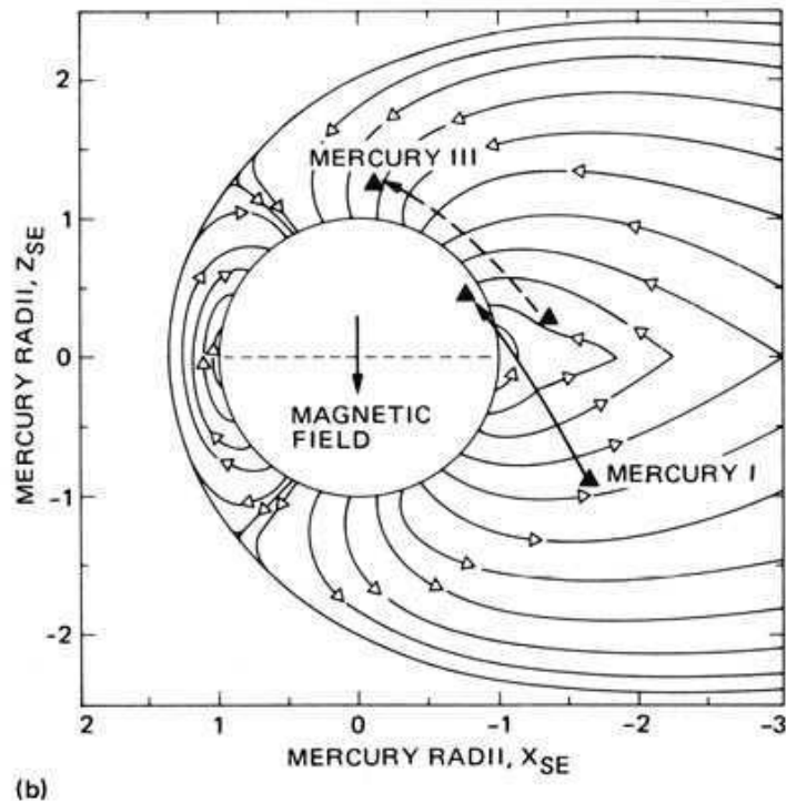
Fig. 8-11. Mariner 10's path through the third encounter passed over the planet. Looking down from the north, (a) shows the interaction of the solar wind with the magnetic field of the planet. The crossings of the bow shock wave and the magnetopause corresponded with the times predicted from the measurements made during the first encounter, thereby confirming that the magnetic field of Mercury is intrinsic to the planet. An equatorial plane view of the planet's magnetic field lines is given in (b), which shows portions of the path of Mariner 10 through the field at the first and third encounters.
