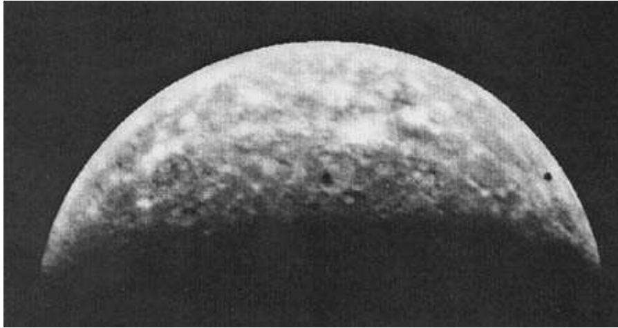
Fig. 7-4. Soon craters on Mercury were positively identified for the first time. Many astronomers had suggested that Mercury would be cratered like the Moon. This computer-enhanced view was taken March 27 from a distance of 1,840,000 km (1,141,000 mi). Craters as small as 160 km (100 mi) across can be made out along the right edge of the crescent, where the Sun is setting on the planet. North is at the top.
