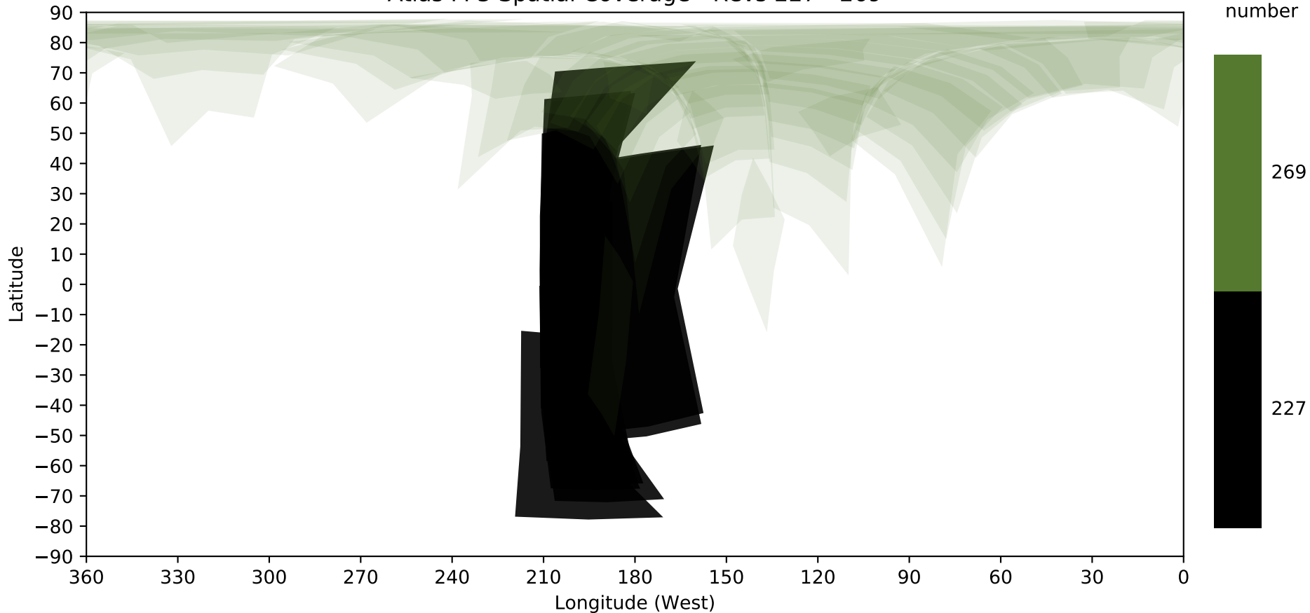
Atlas FP3 Spatial Coverage - Revs 227 - 269
