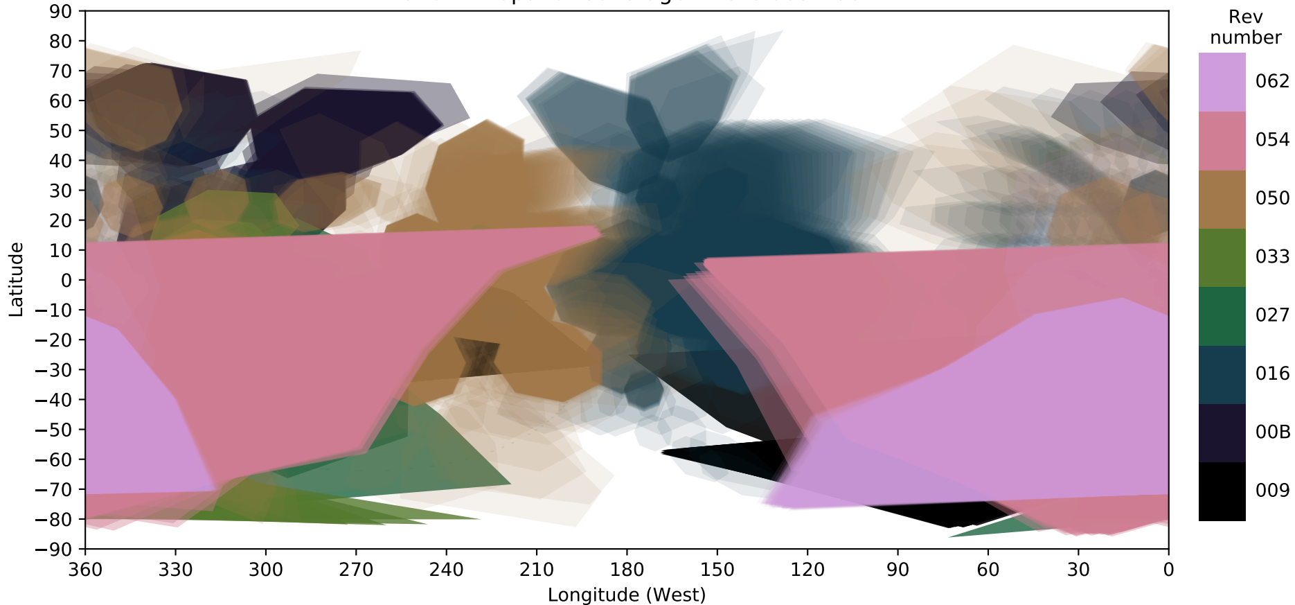
Dione FP1 Spatial Coverage - Revs 009 - 062
