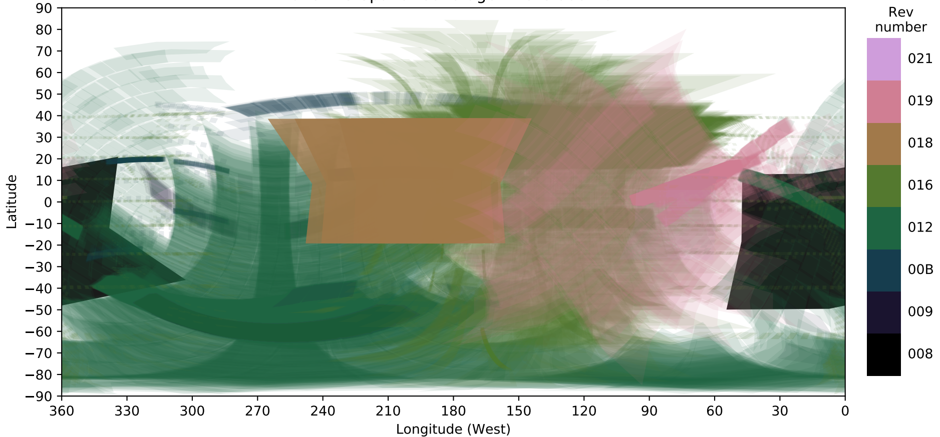
Dione FP3 Spatial Coverage - Revs 008 - 021
