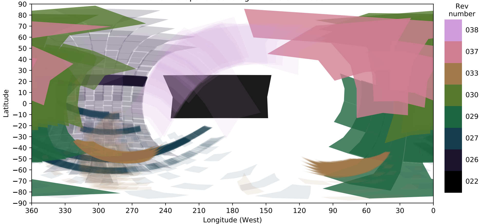
Dione FP3 Spatial Coverage - Revs 022 - 038
