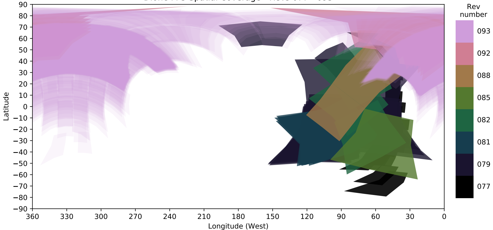
Dione FP3 Spatial Coverage - Revs 077 - 093
