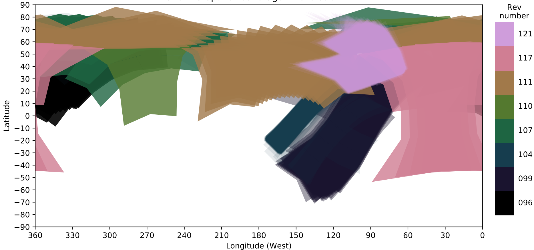
Dione FP3 Spatial Coverage - Revs 096 - 121
