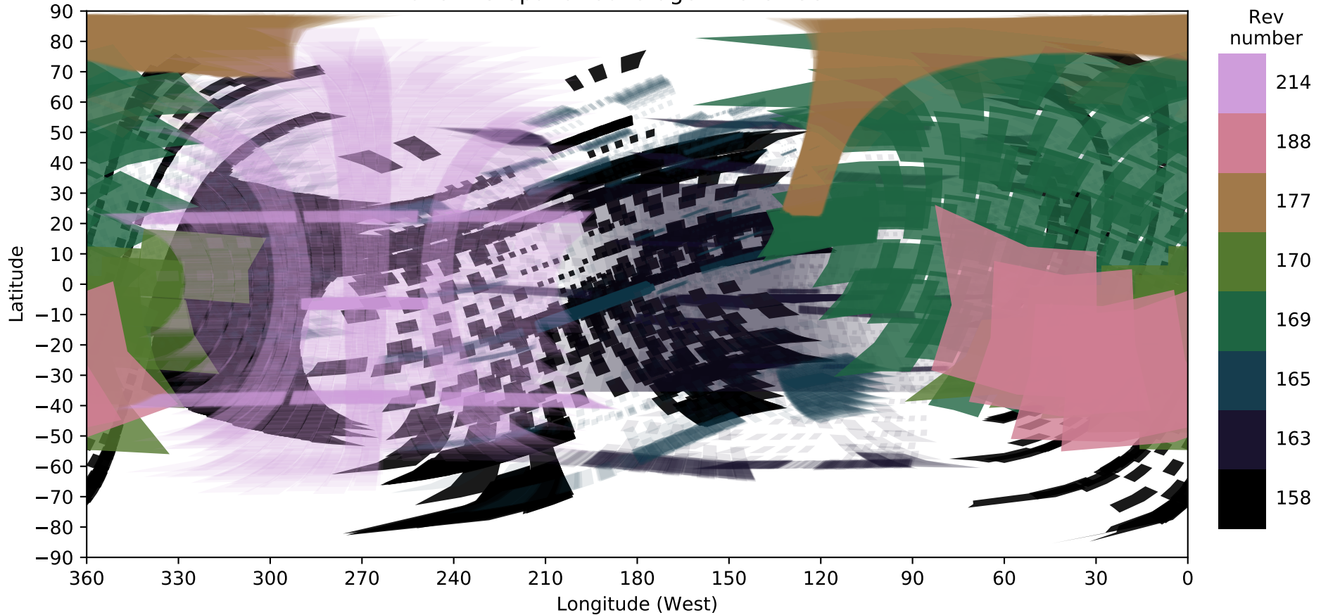
Dione FP3 Spatial Coverage - Revs 158 - 214
