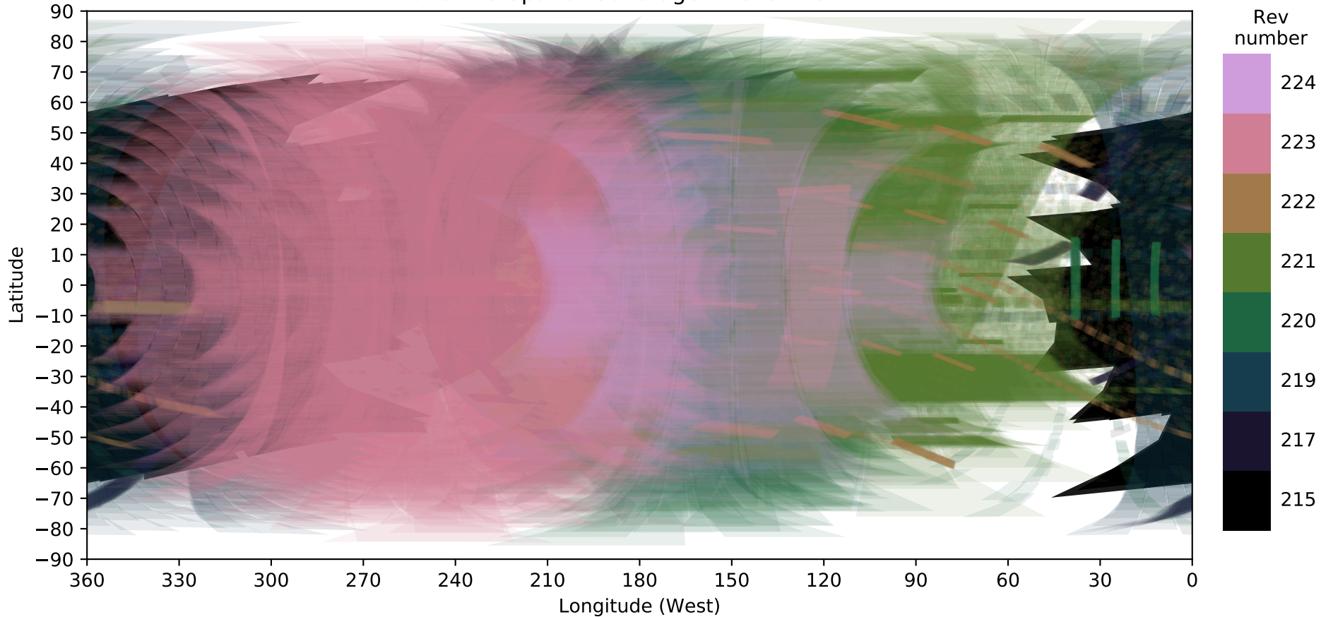
Dione FP3 Spatial Coverage - Revs 215 - 224
