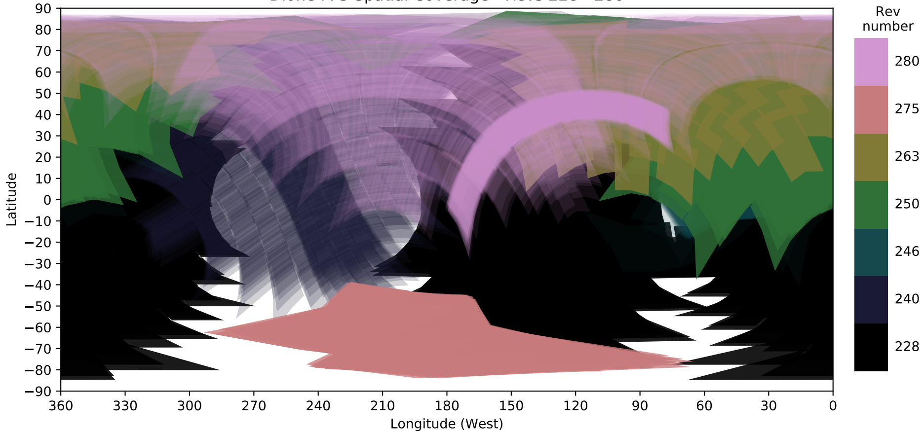
Dione FP3 Spatial Coverage - Revs 228 - 280
