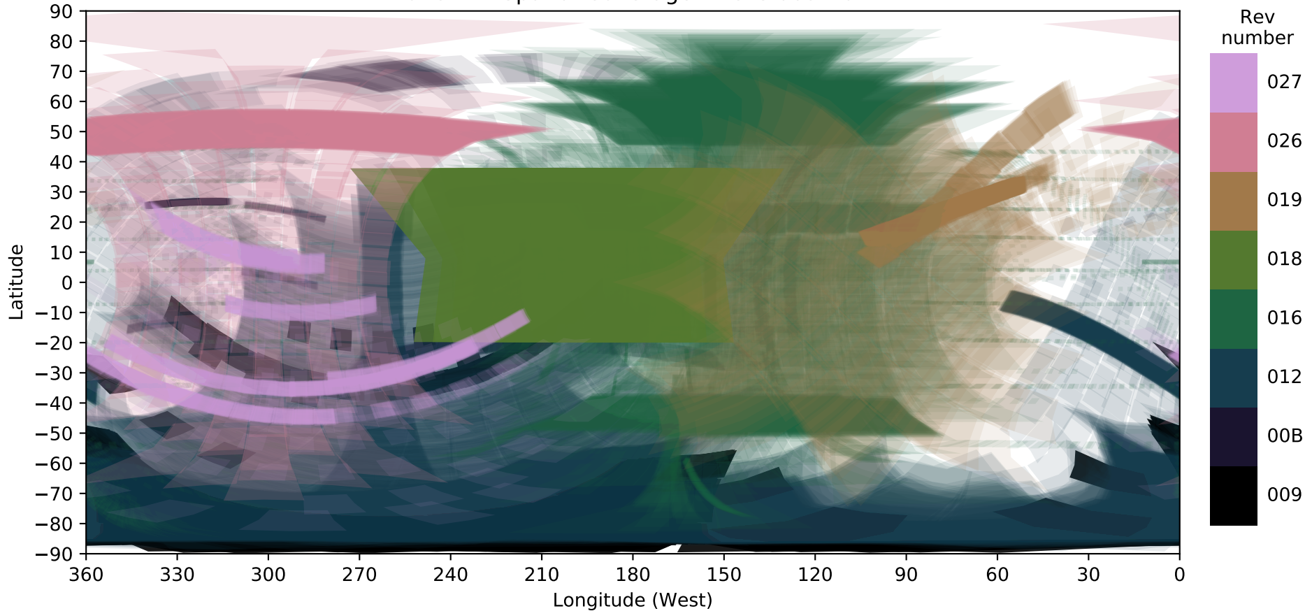
Dione FP4 Spatial Coverage - Revs 009 - 027
