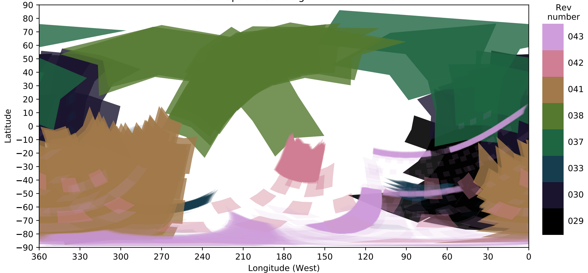
Dione FP4 Spatial Coverage - Revs 029 - 043
