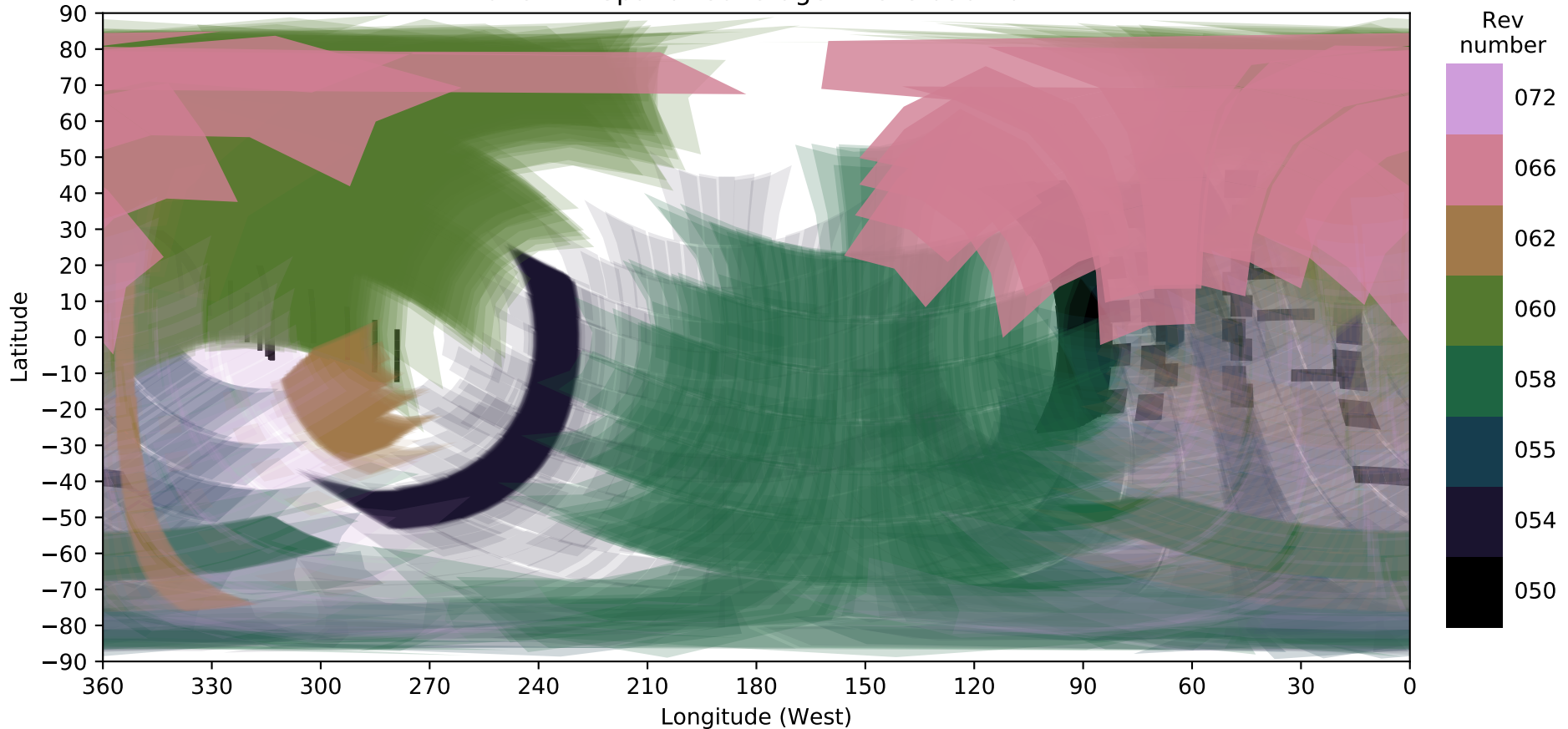
Dione FP4 Spatial Coverage - Revs 050 - 072
