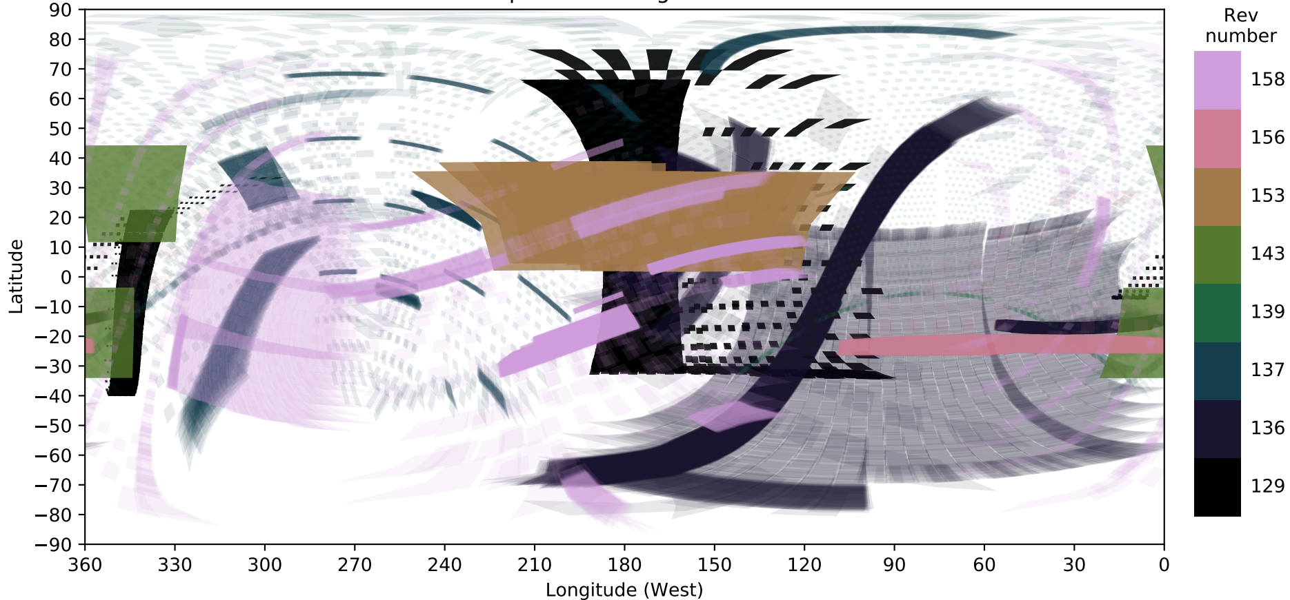
Dione FP4 Spatial Coverage - Revs 129 - 158
