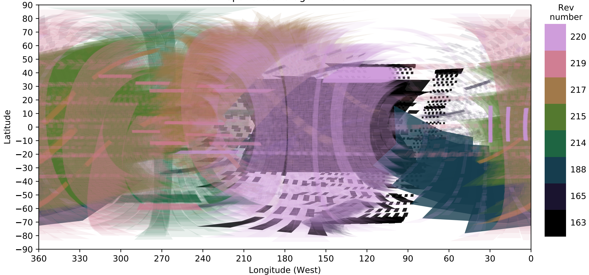
Dione FP4 Spatial Coverage - Revs 163 - 220
