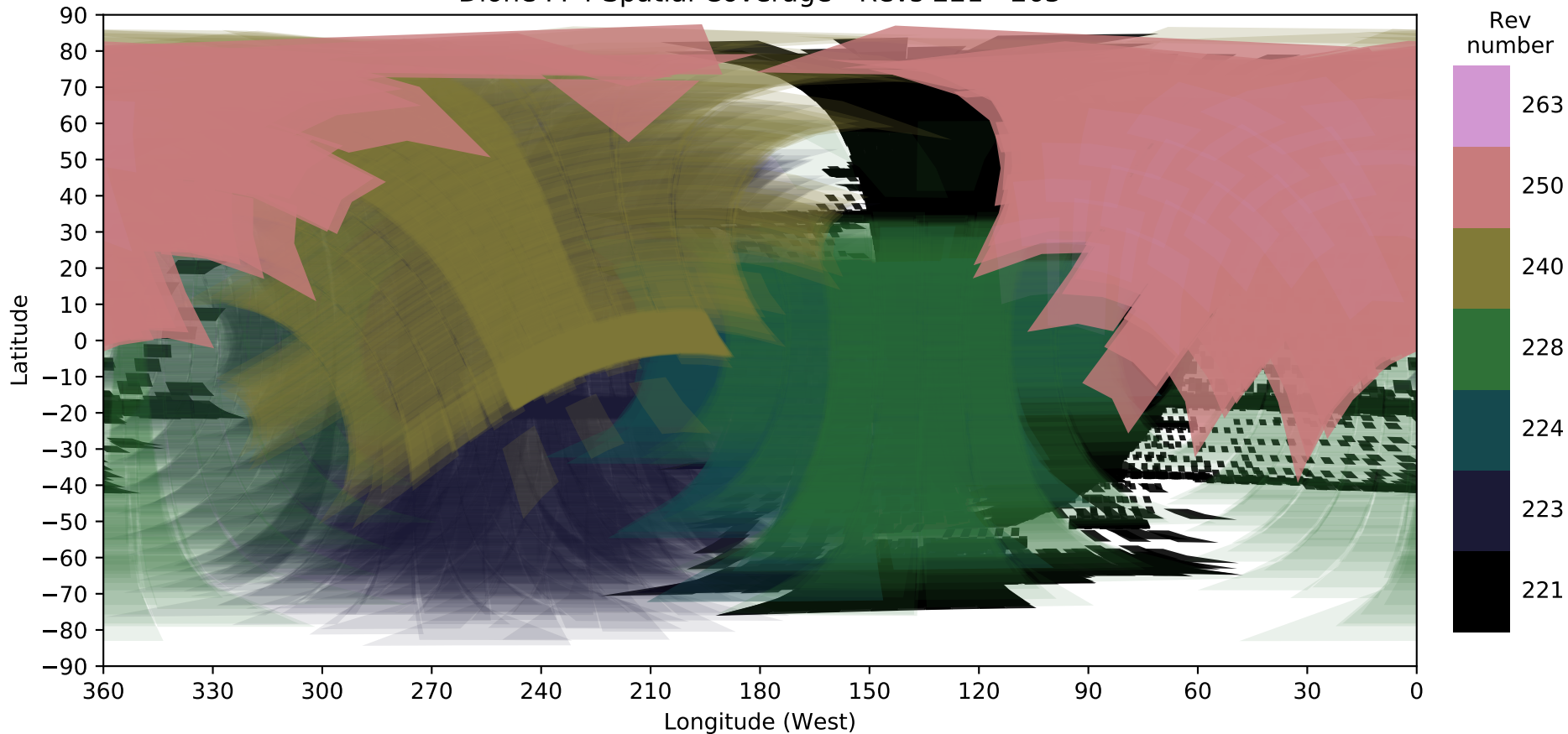
Dione FP4 Spatial Coverage - Revs 221 - 263
