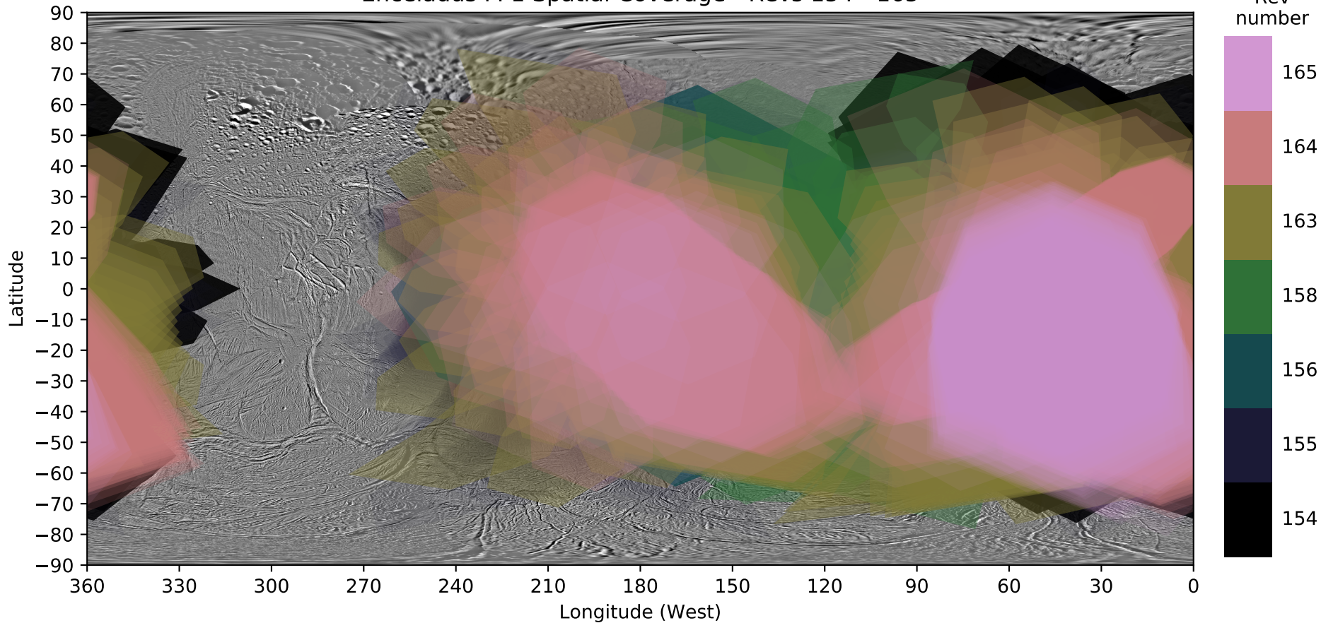
Enceladus FP1 Spatial Coverage - Revs 154 - 165
