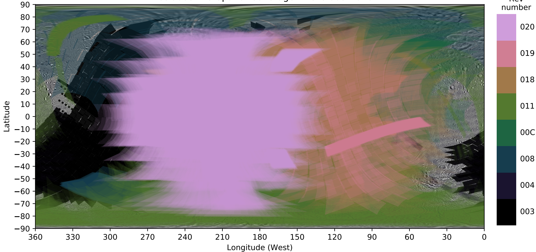
Enceladus FP3 Spatial Coverage - Revs 003 - 020
