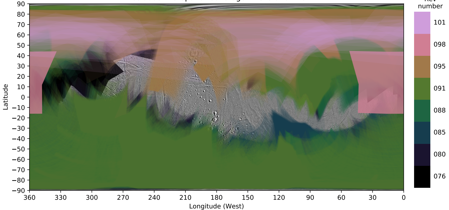
Enceladus FP3 Spatial Coverage - Revs 076 - 101
