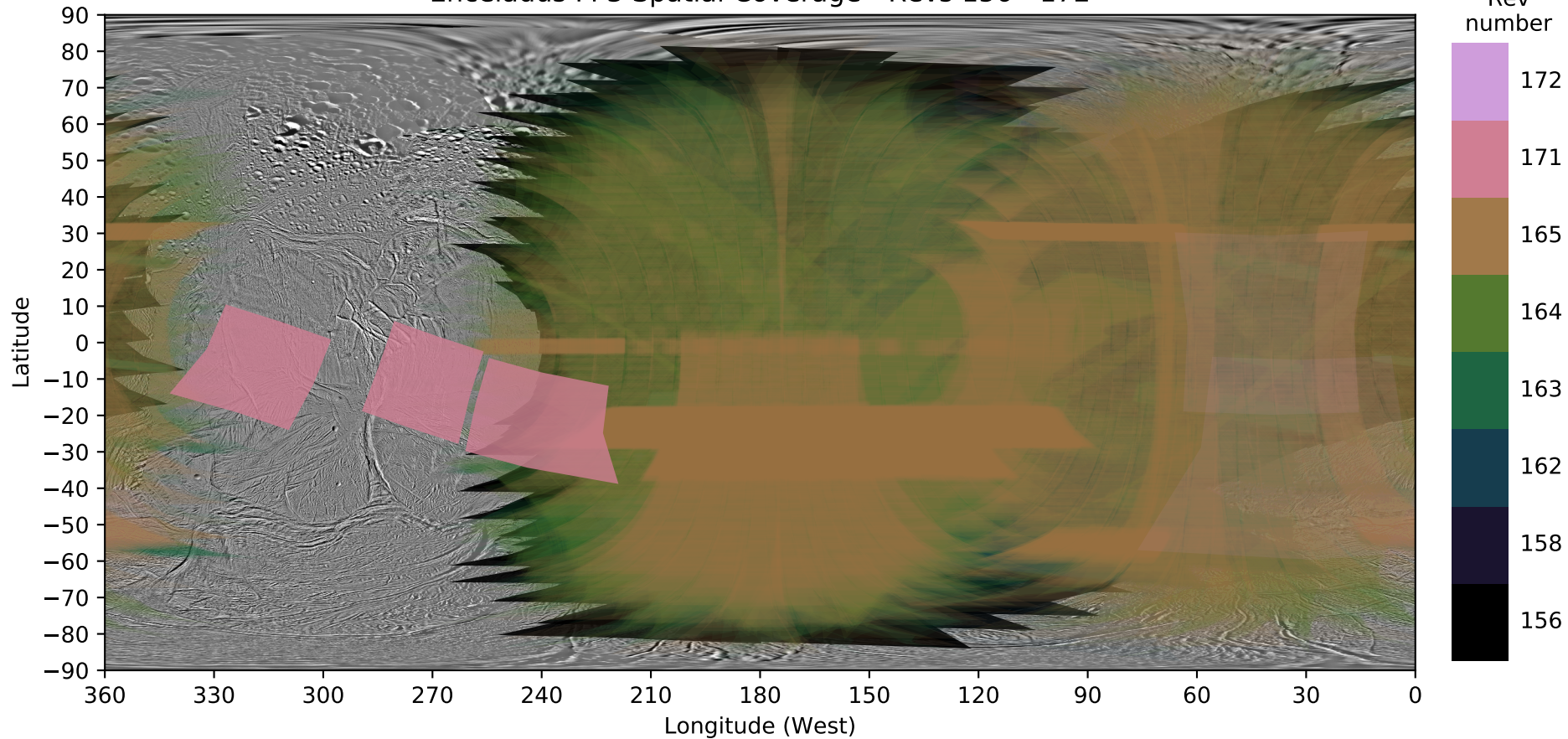
Enceladus FP3 Spatial Coverage - Revs 156 - 172
