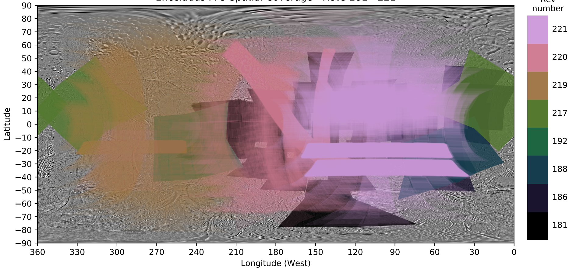
Enceladus FP3 Spatial Coverage - Revs 181 - 221
