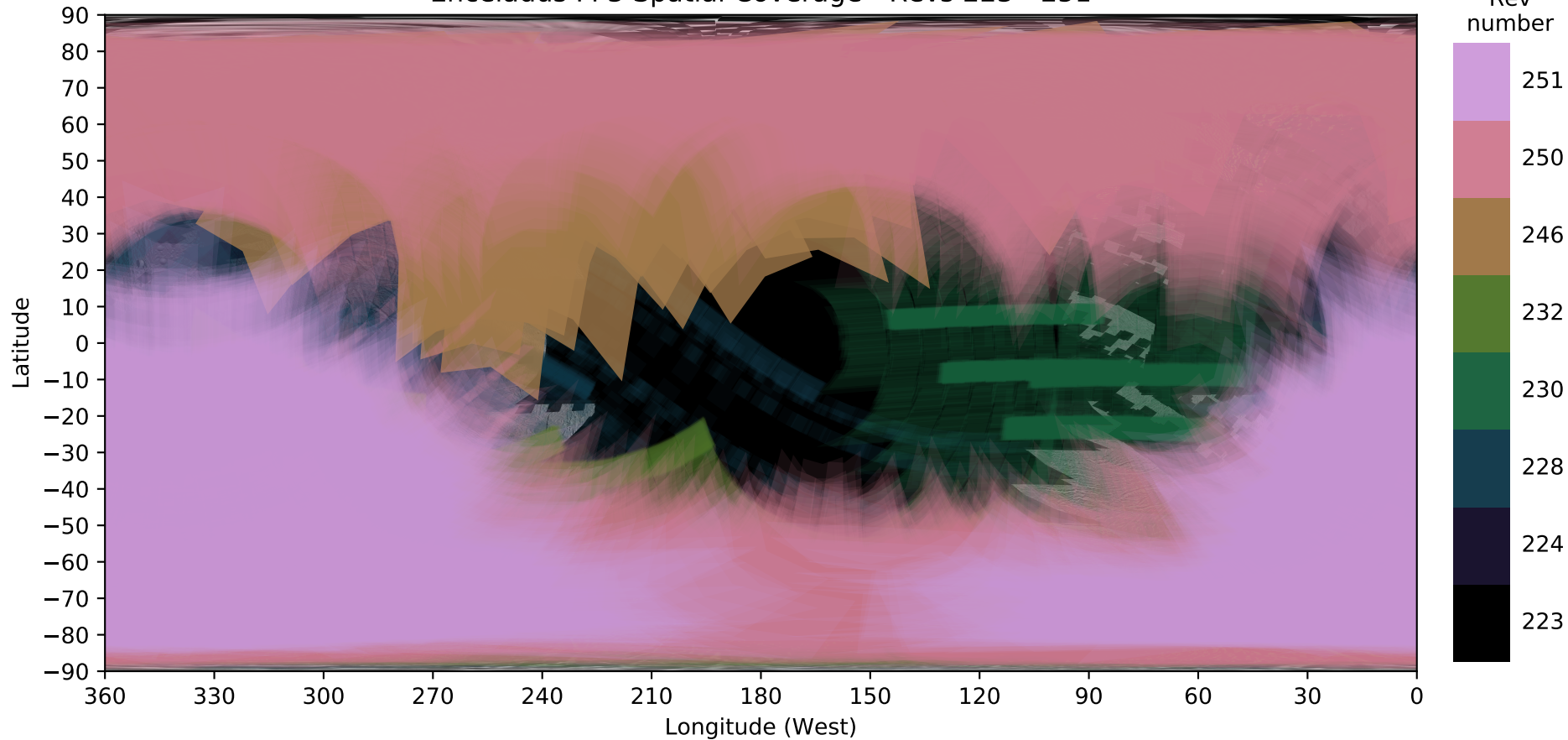
Enceladus FP3 Spatial Coverage - Revs 223 - 251
