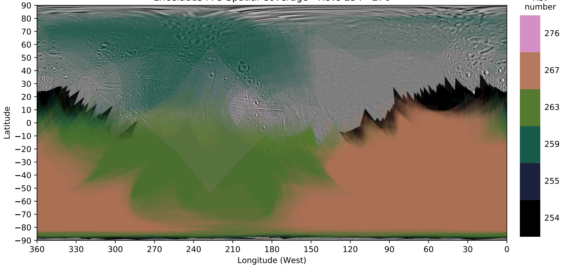
Enceladus FP3 Spatial Coverage - Revs 254 - 276
