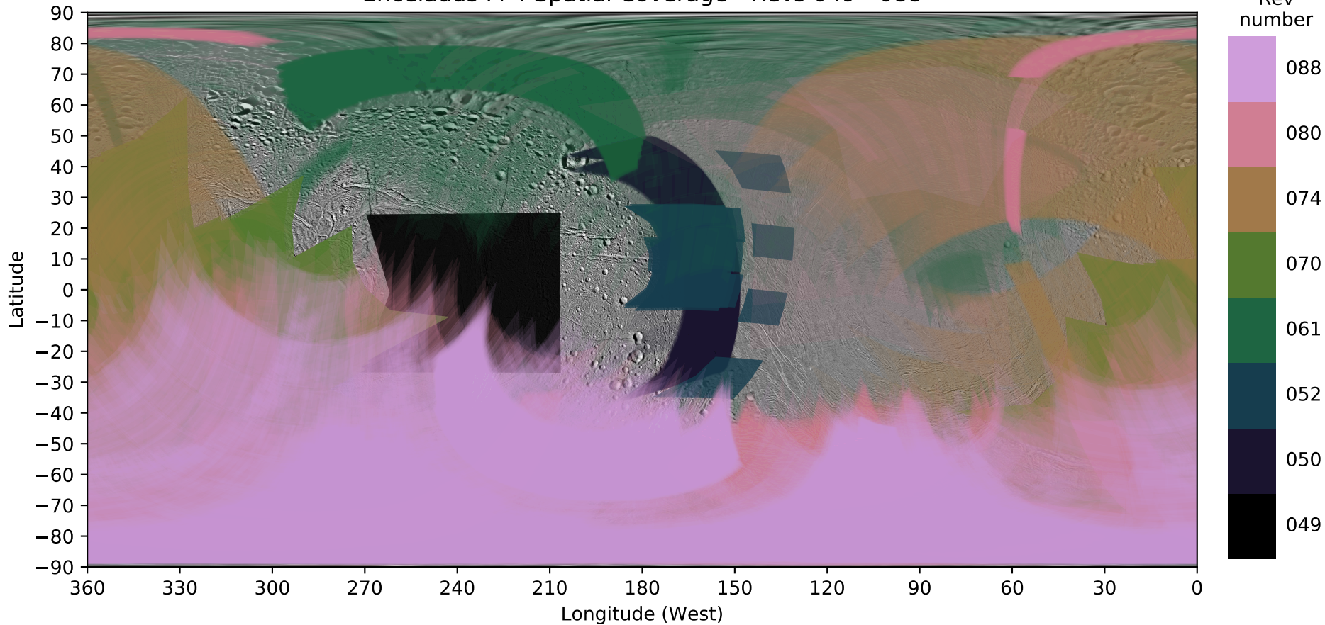
Enceladus FP4 Spatial Coverage - Revs 049 - 088
