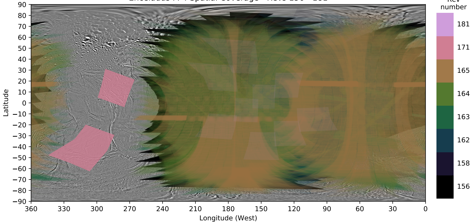
Enceladus FP4 Spatial Coverage - Revs 156 - 181
