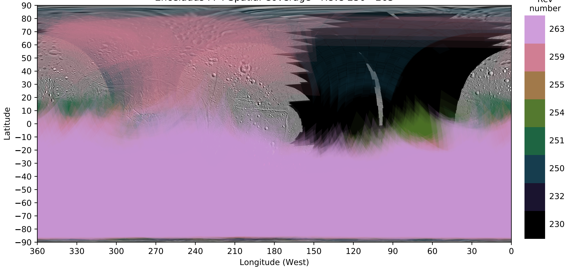
Enceladus FP4 Spatial Coverage - Revs 230 - 263
