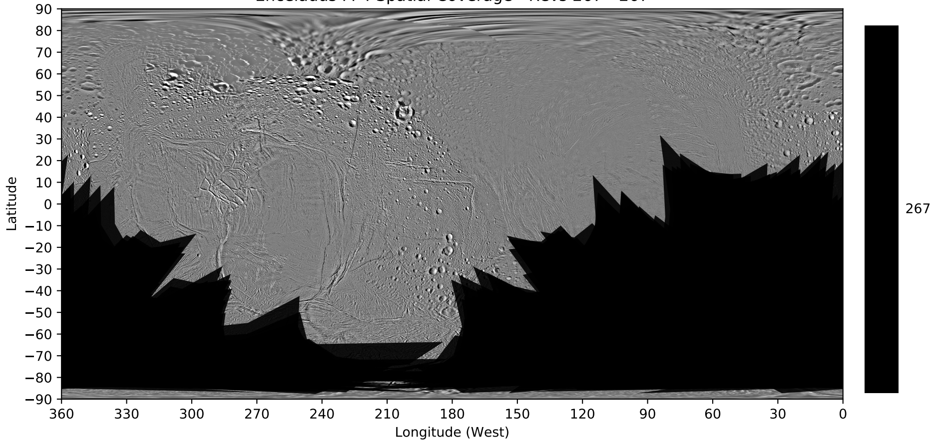
Enceladus FP4 Spatial Coverage - Revs 267 - 267
