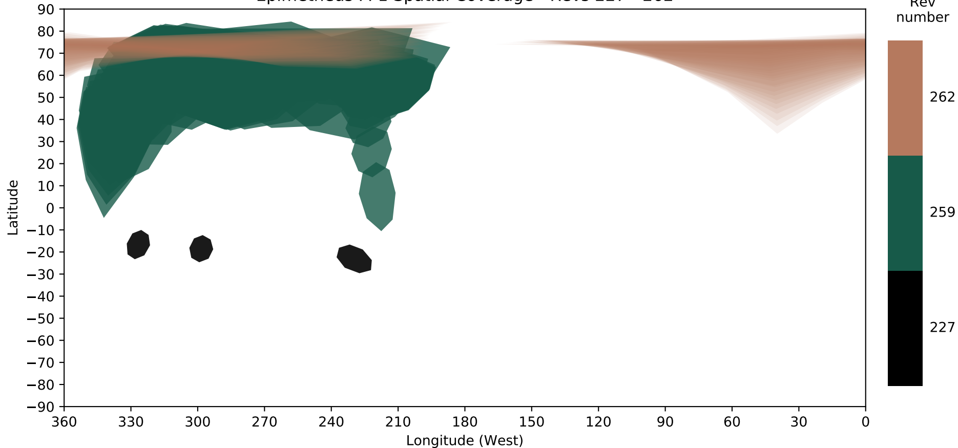
Epimetheus FP1 Spatial Coverage - Revs 227 - 262
