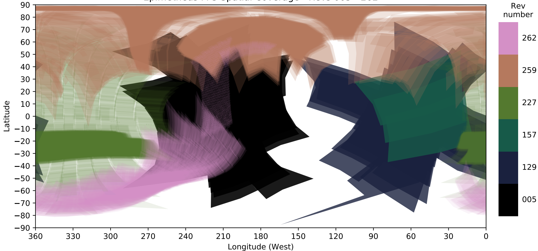
Epimetheus FP3 Spatial Coverage - Revs 005 - 262
