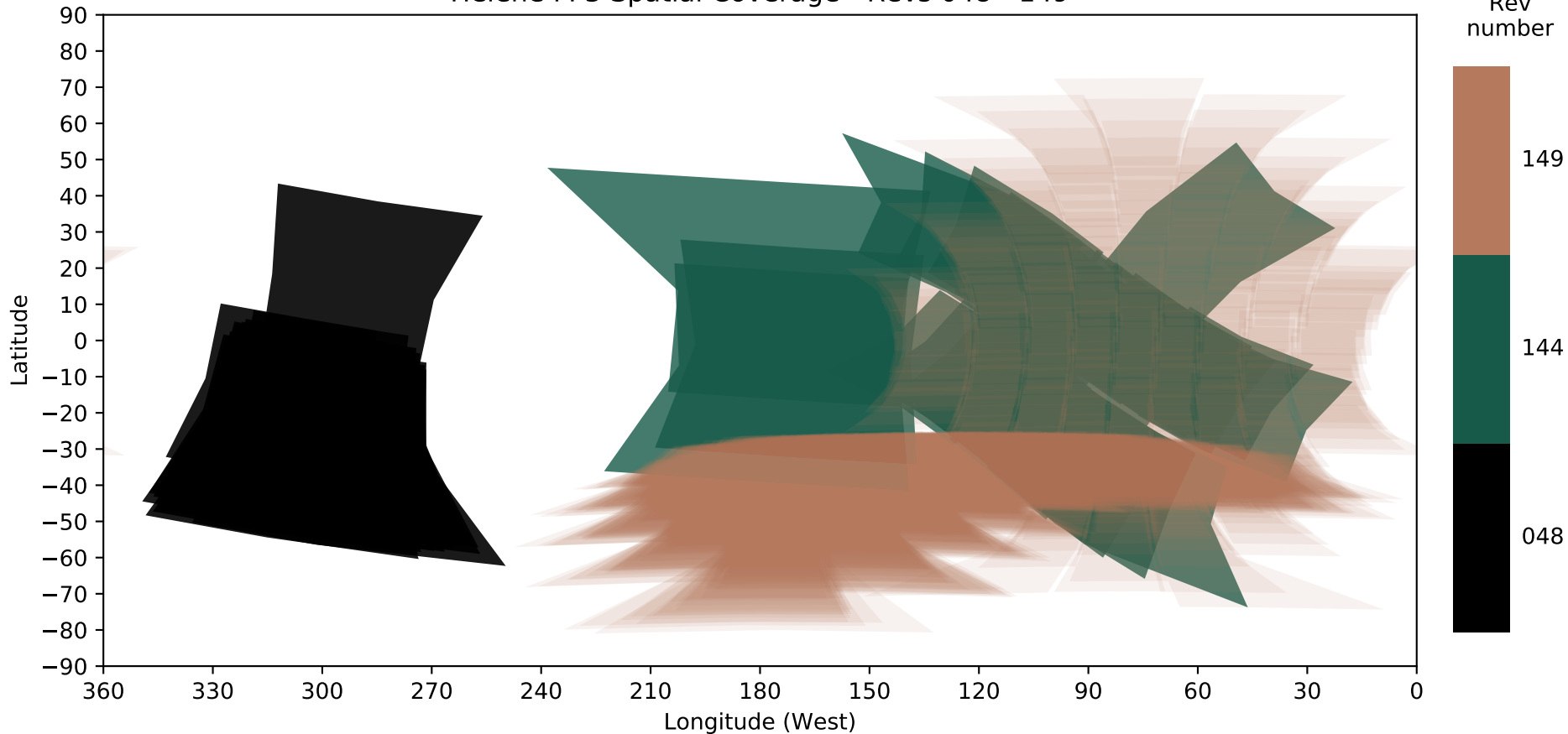
Helene FP3 Spatial Coverage - Revs 048 - 149
