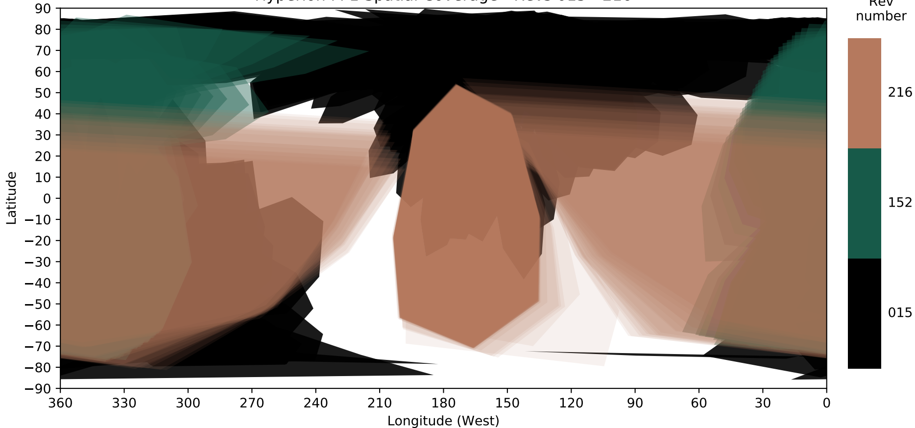
Hyperion FP1 Spatial Coverage - Revs 015 - 216
