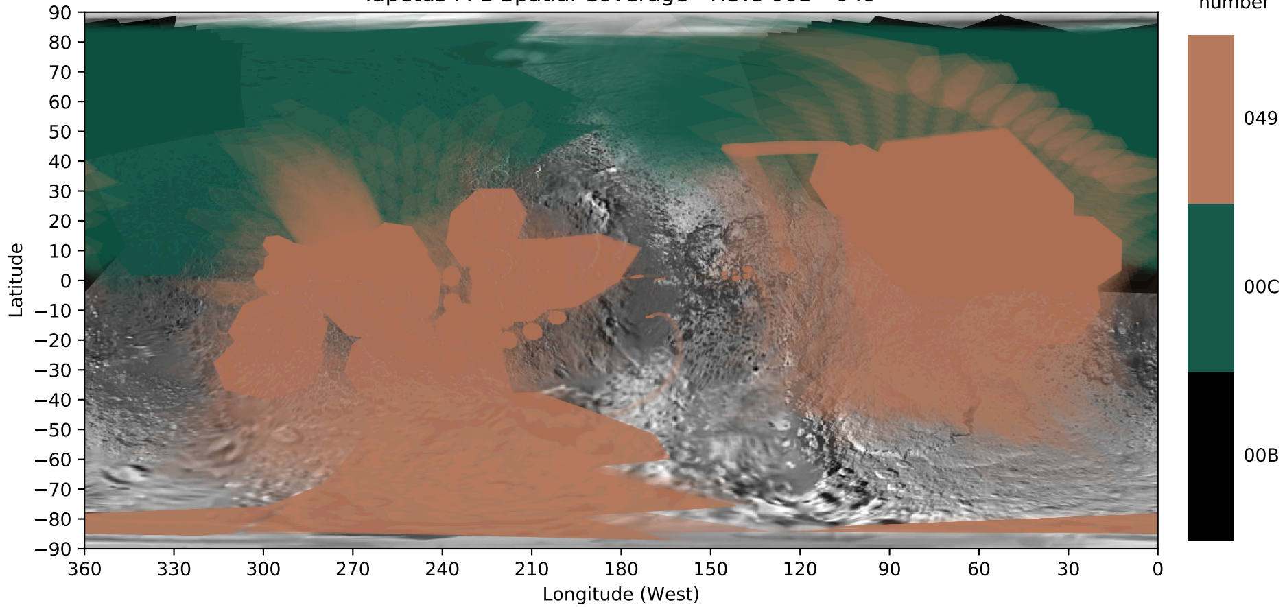
Iapetus FP1 Spatial Coverage - Revs 00B - 049
