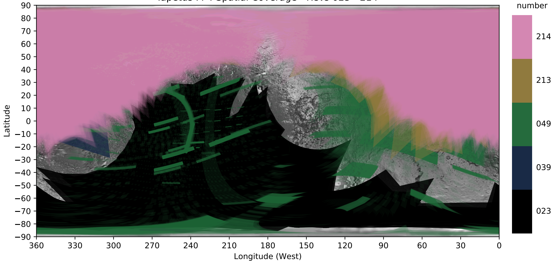
Iapetus FP4 Spatial Coverage - Revs 023 - 214
