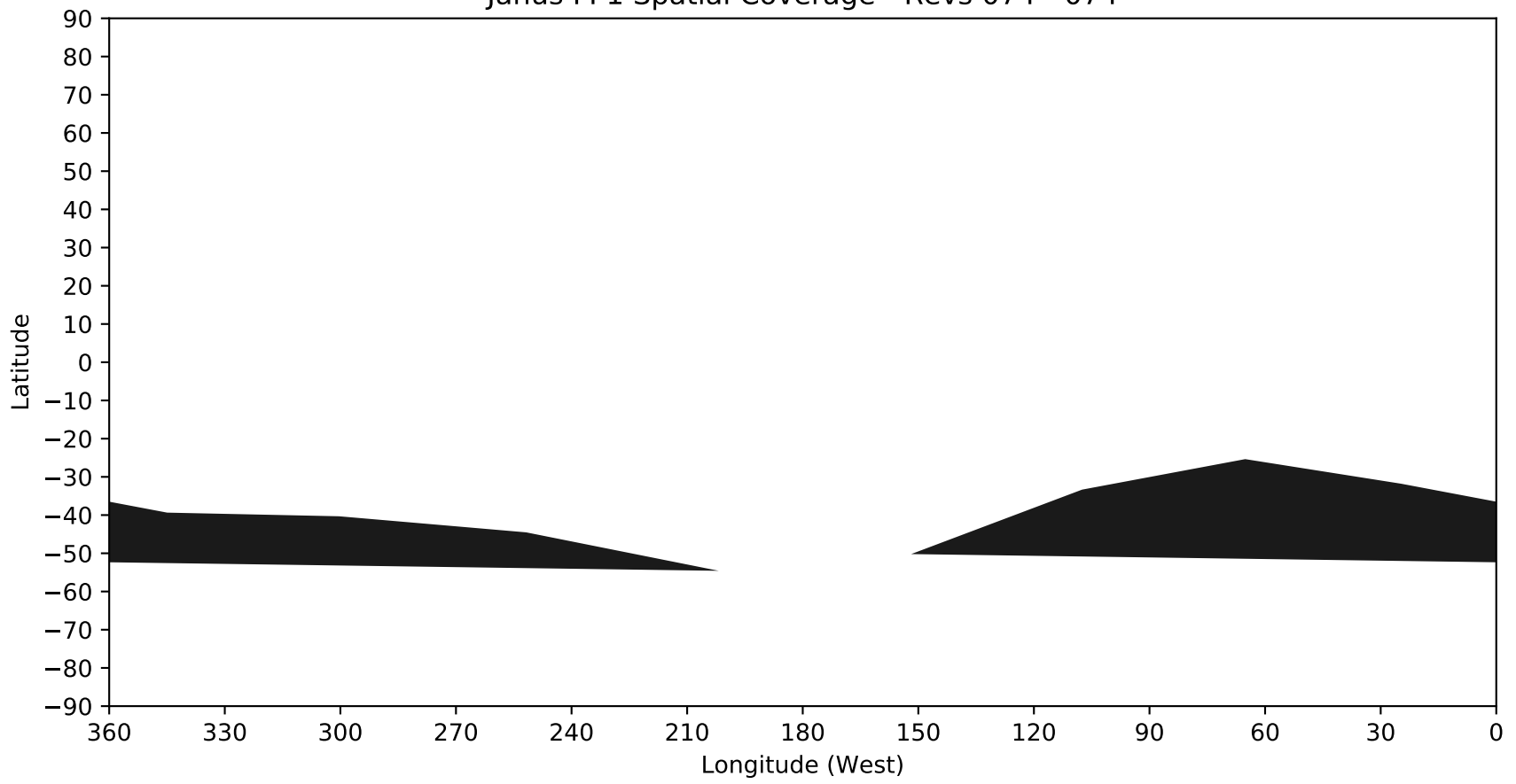
Janus FP1 Spatial Coverage - Revs 074 - 074
