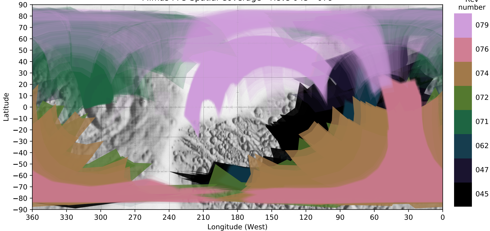
Mimas FP3 Spatial Coverage - Revs 045 - 079
