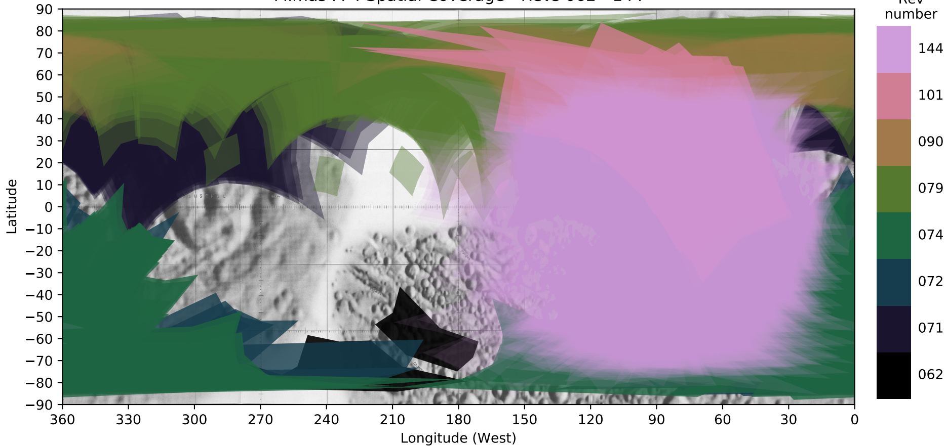
Mimas FP4 Spatial Coverage - Revs 062 - 144
