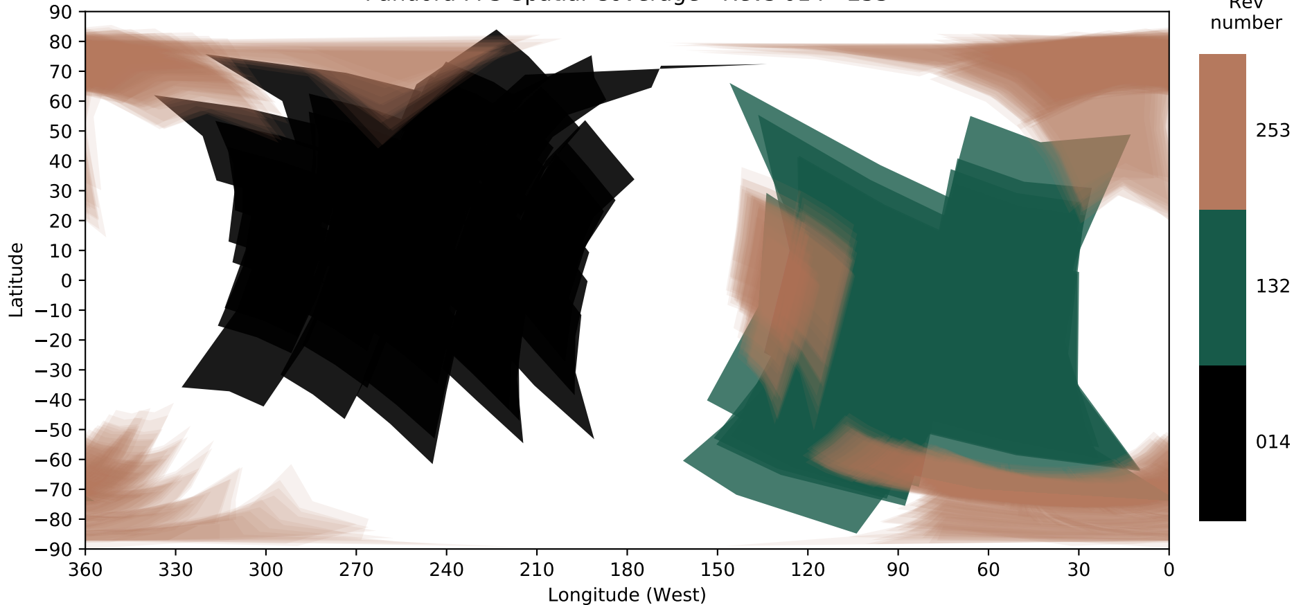
Pandora FP3 Spatial Coverage - Revs 014 - 253
