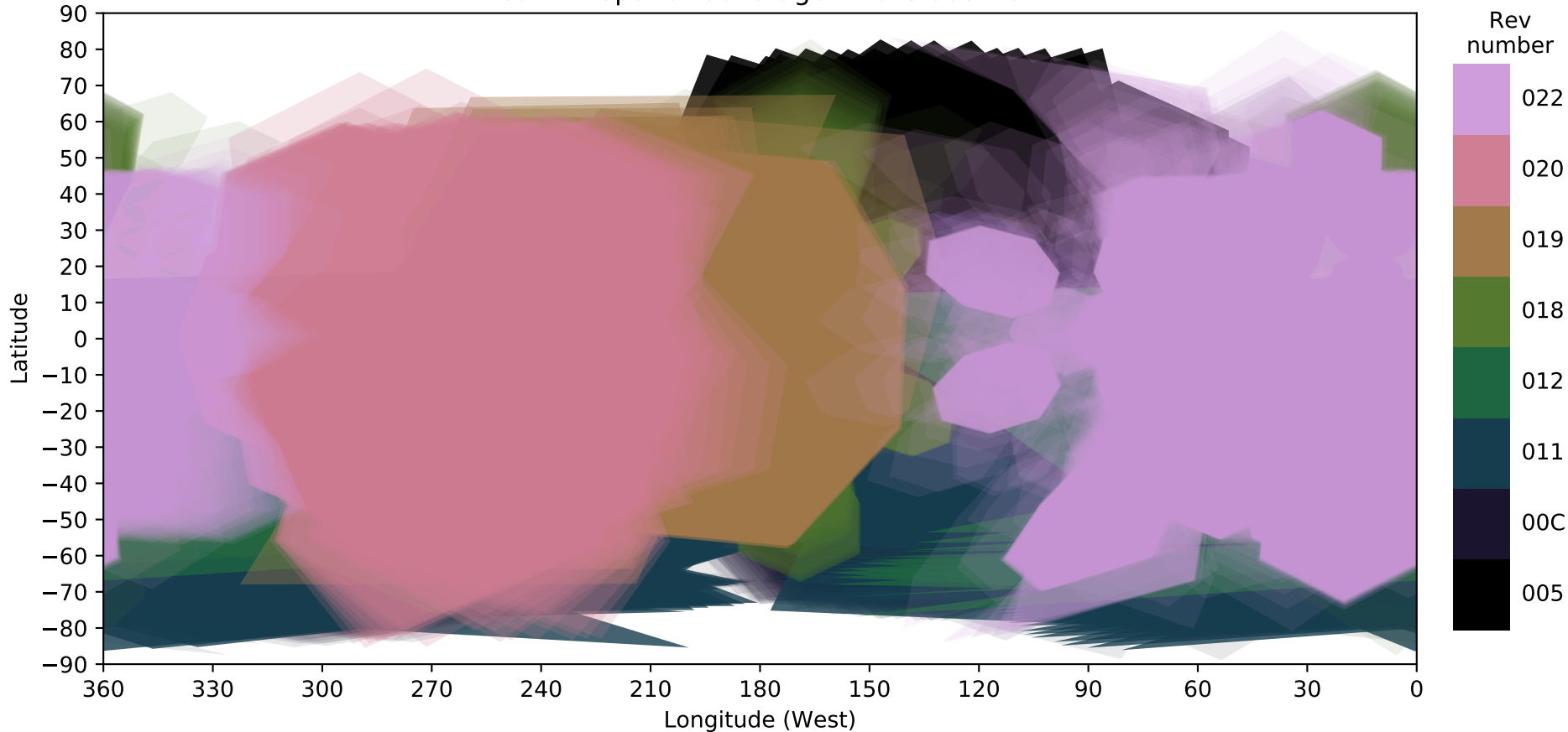
Rhea FP1 Spatial Coverage - Revs 005 - 022
