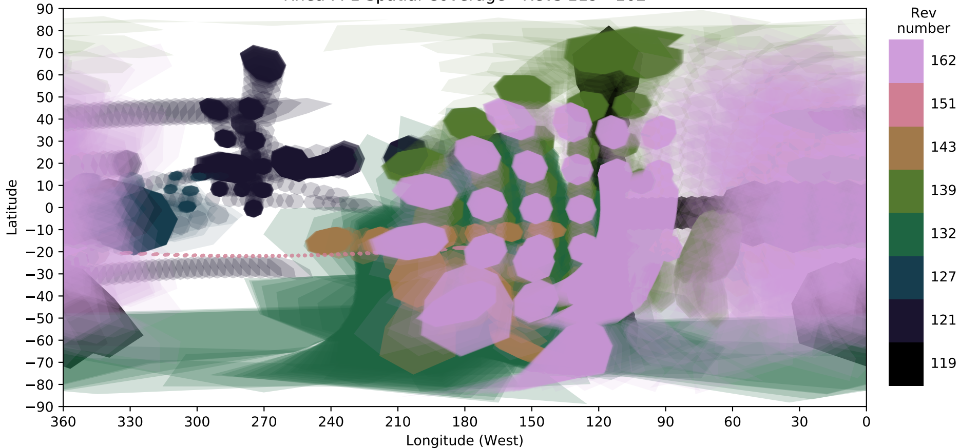
Rhea FP1 Spatial Coverage - Revs 119 - 162
