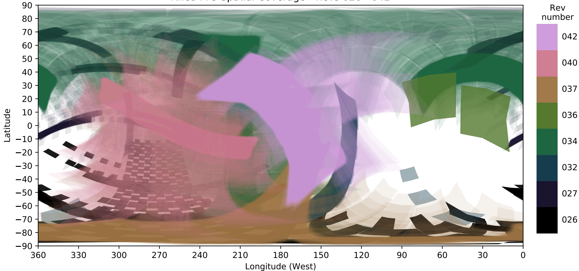
Rhea FP3 Spatial Coverage - Revs 026 - 042
