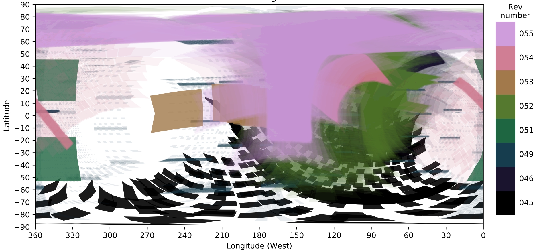
Rhea FP3 Spatial Coverage - Revs 045 - 055
