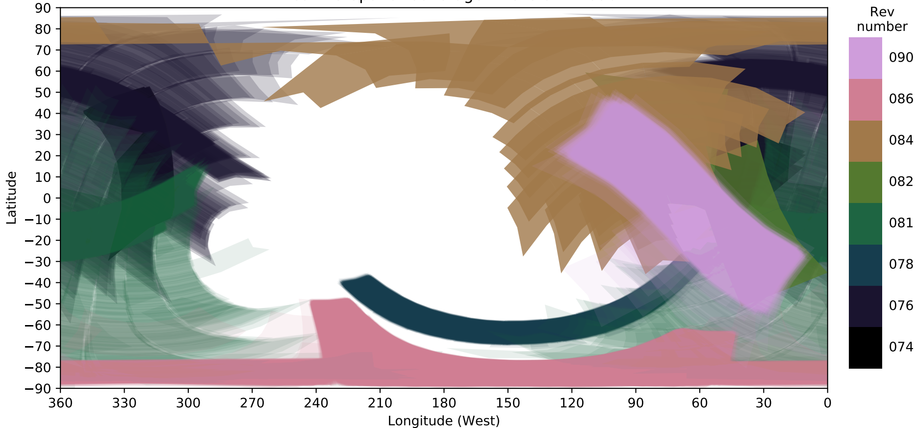
Rhea FP3 Spatial Coverage - Revs 074 - 090
