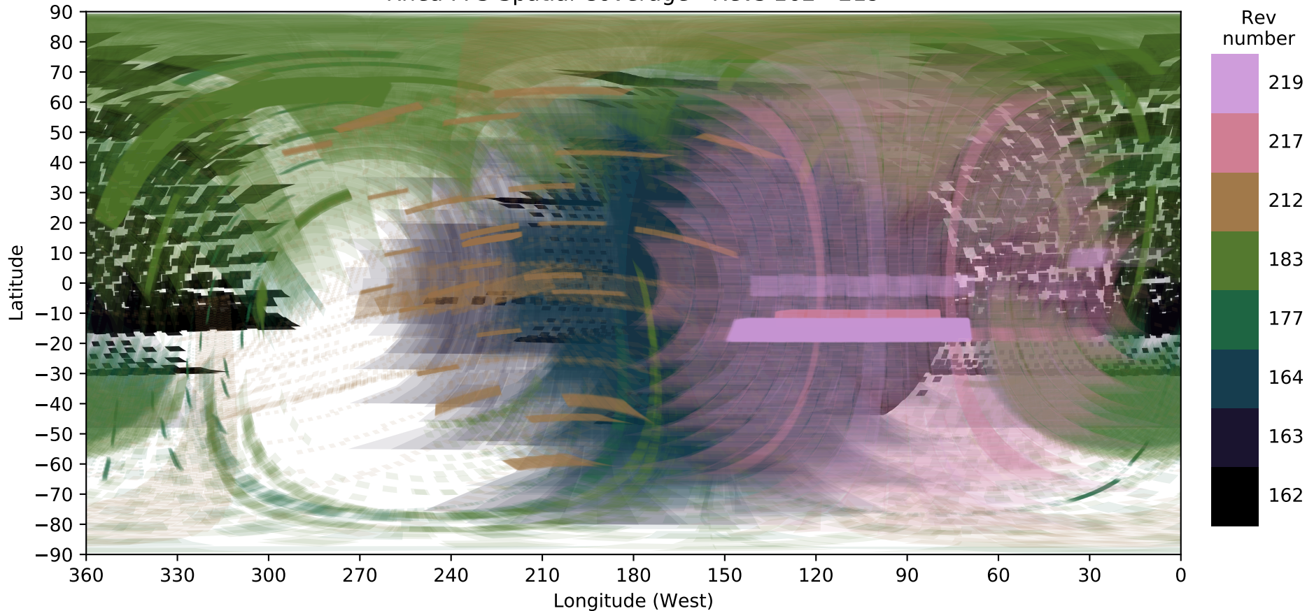
Rhea FP3 Spatial Coverage - Revs 162 - 219
