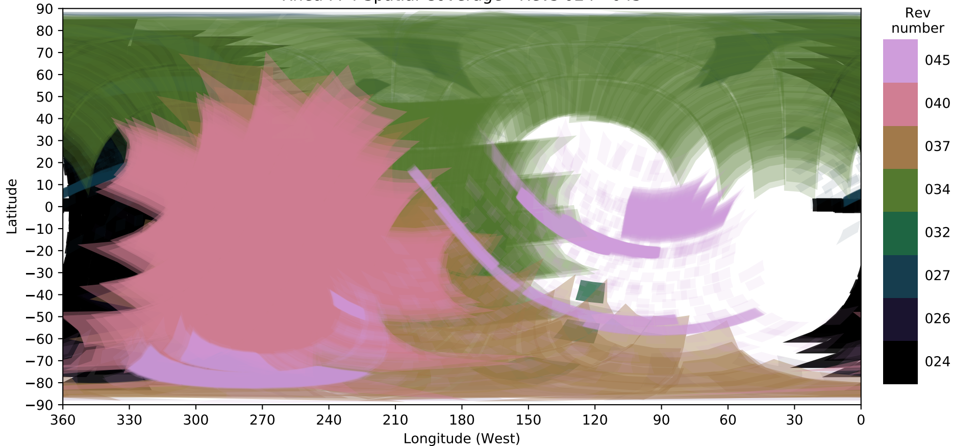
Rhea FP4 Spatial Coverage - Revs 024 - 045
