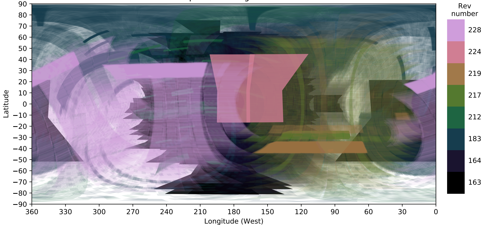
Rhea FP4 Spatial Coverage - Revs 163 - 228
