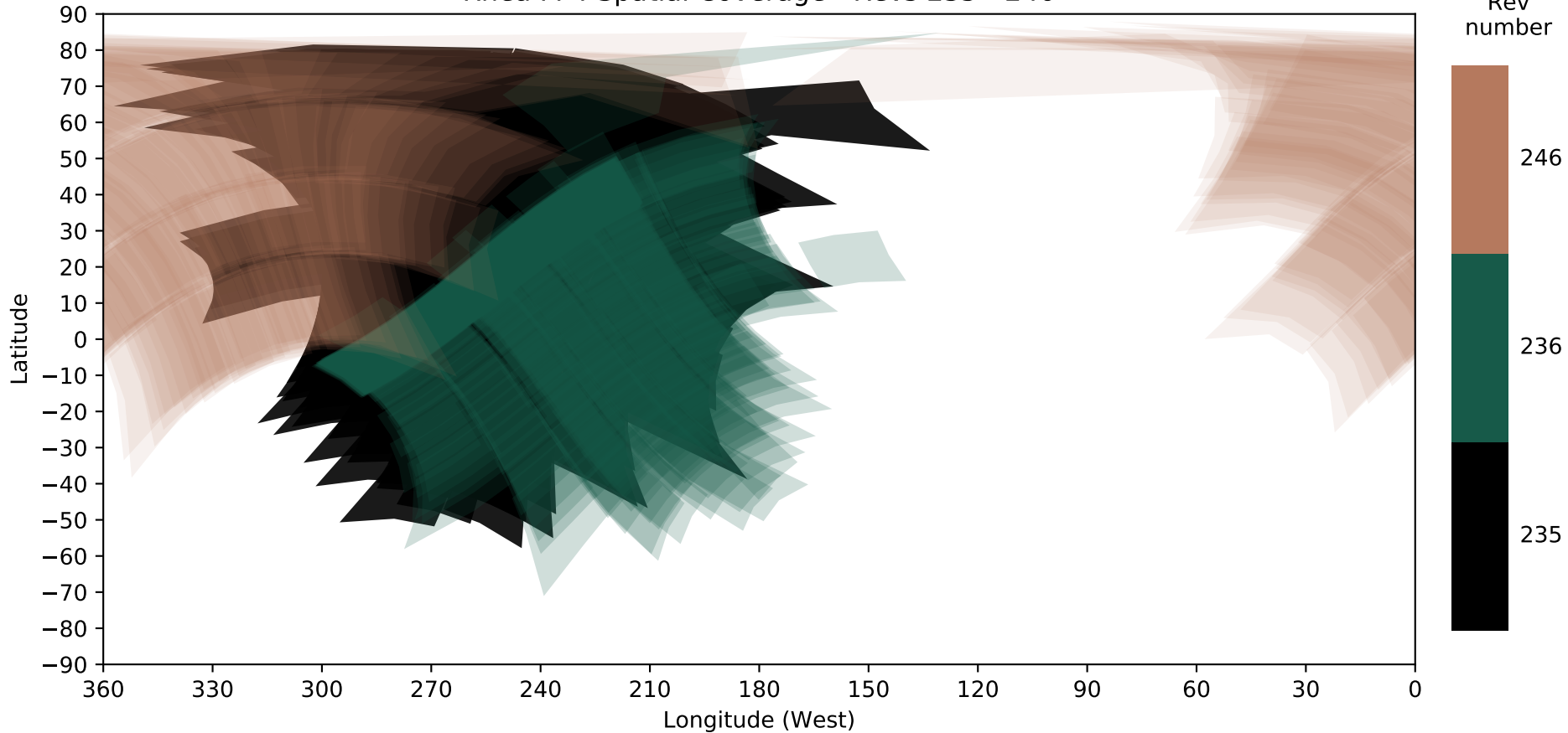
Rhea FP4 Spatial Coverage - Revs 235 - 246
