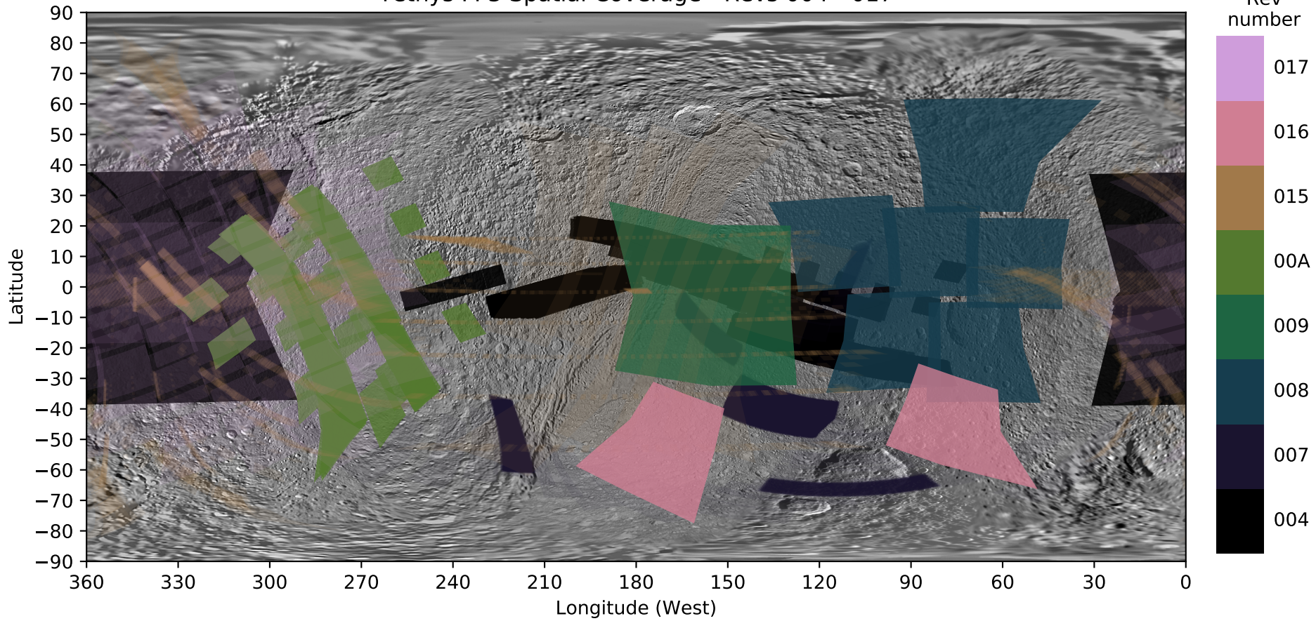
Tethys FP3 Spatial Coverage - Revs 004 - 017
