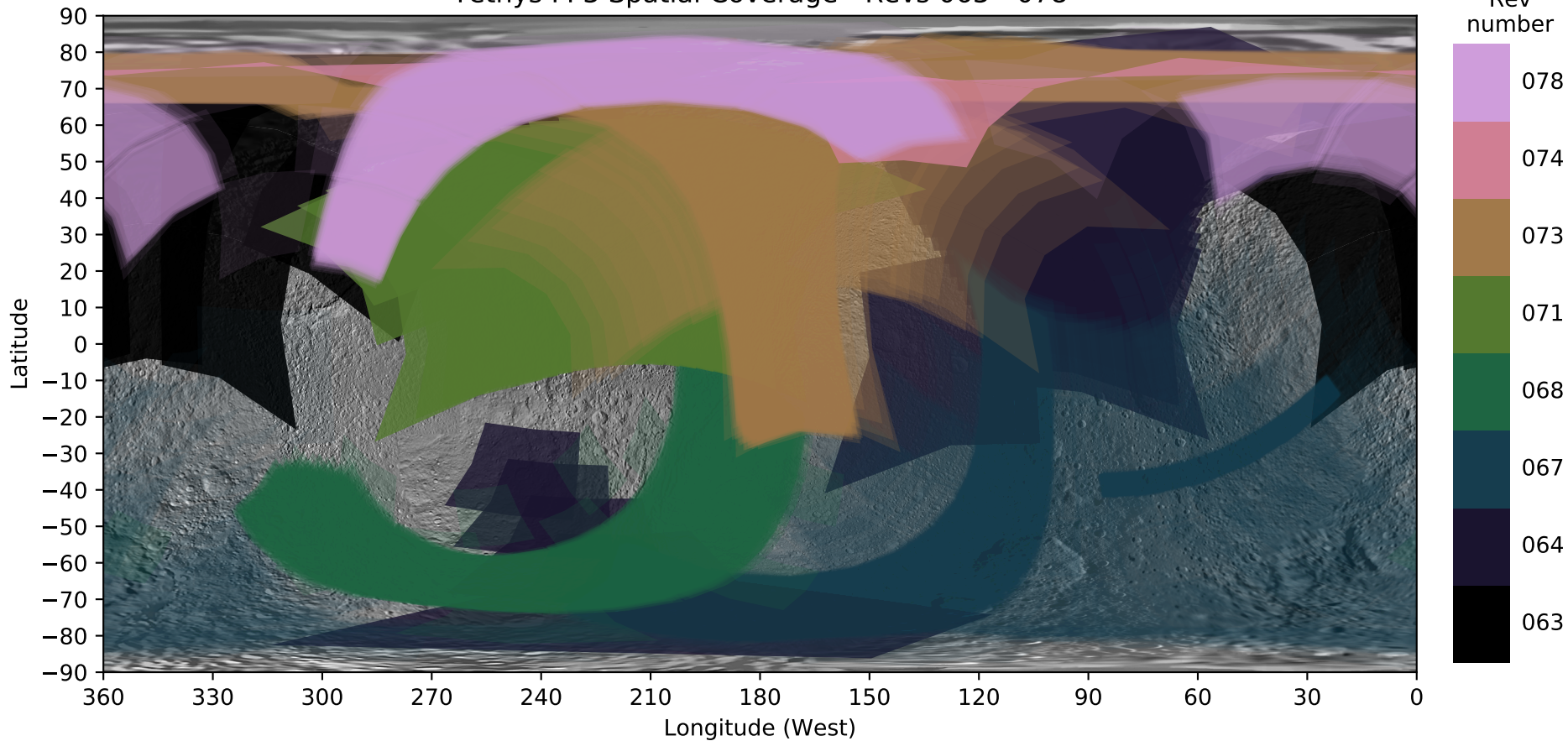
Tethys FP3 Spatial Coverage - Revs 063 - 078
