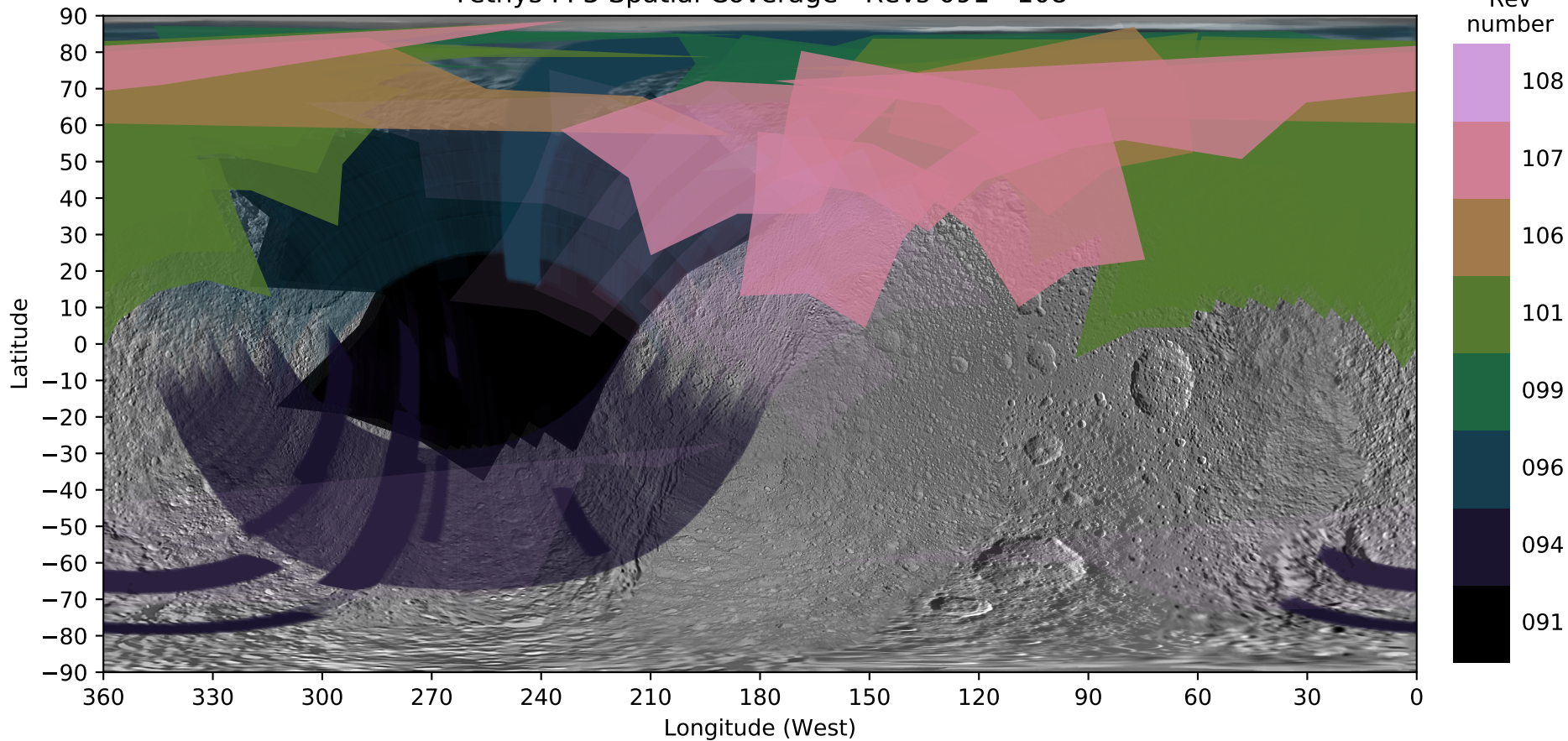
Tethys FP3 Spatial Coverage - Revs 091 - 108
